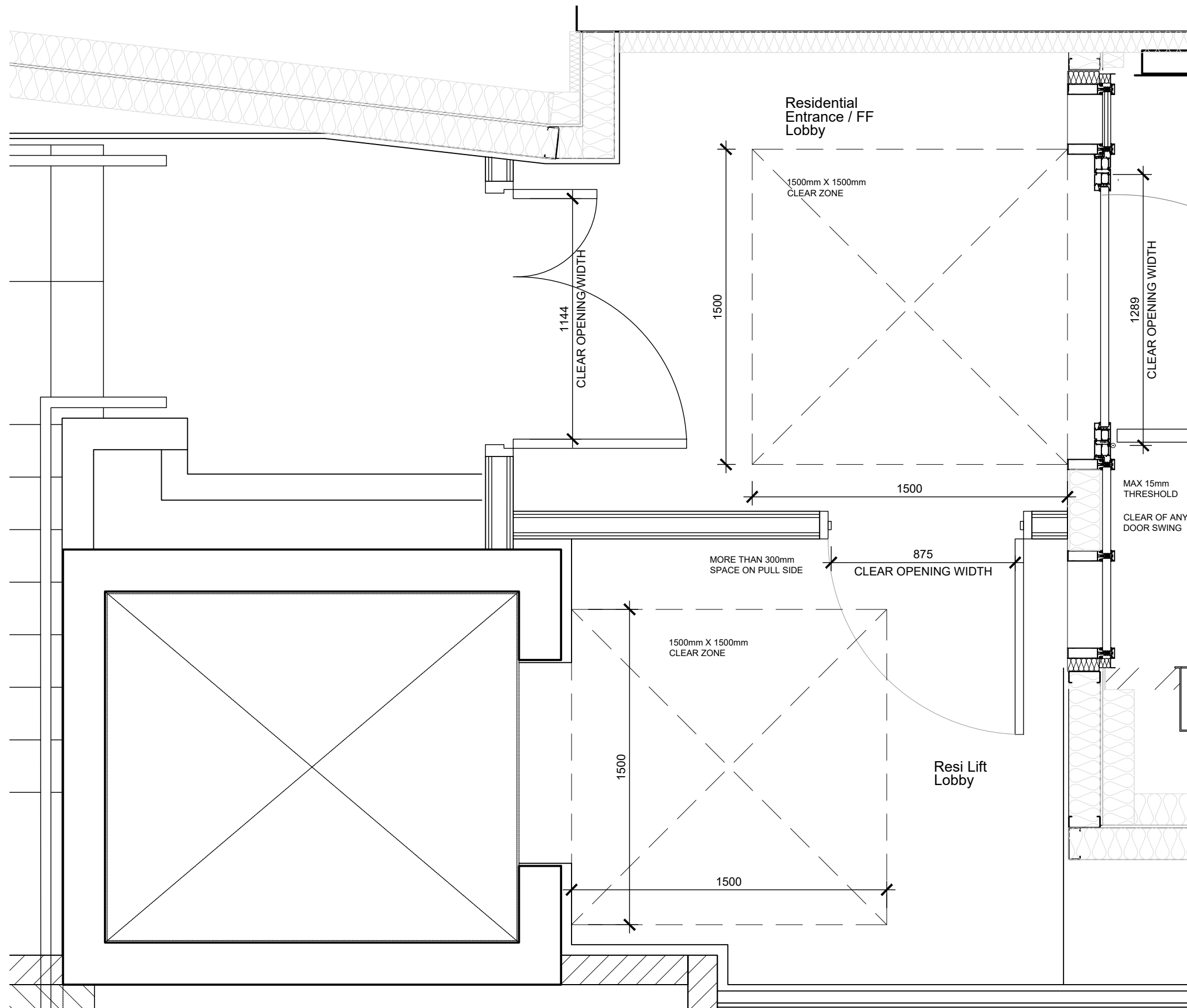
RESIDENTIAL ENTRANCE PLAN - SCALE 1:20
