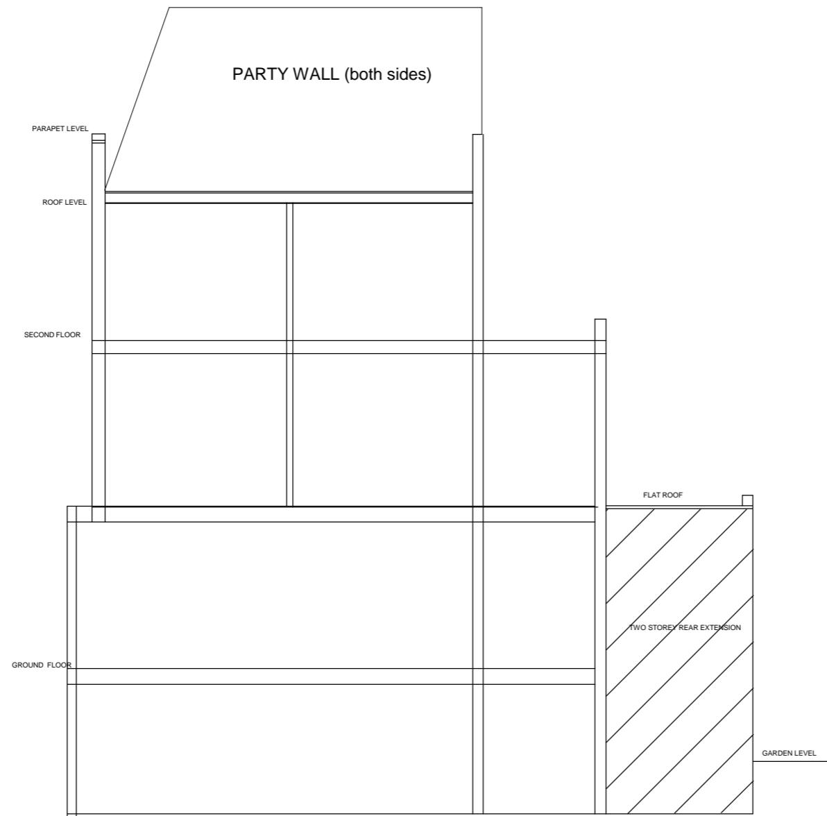
EXISTING LONG SECTION
