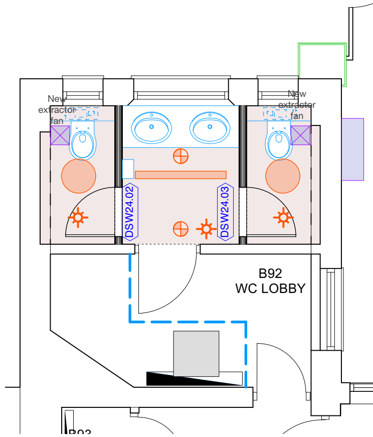
FLOOR PLAN - ROOM B91
