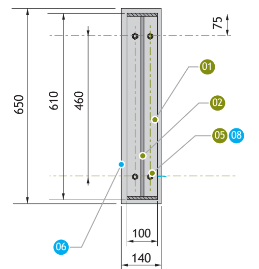
Section through sign frame/ bracket (X-X)
