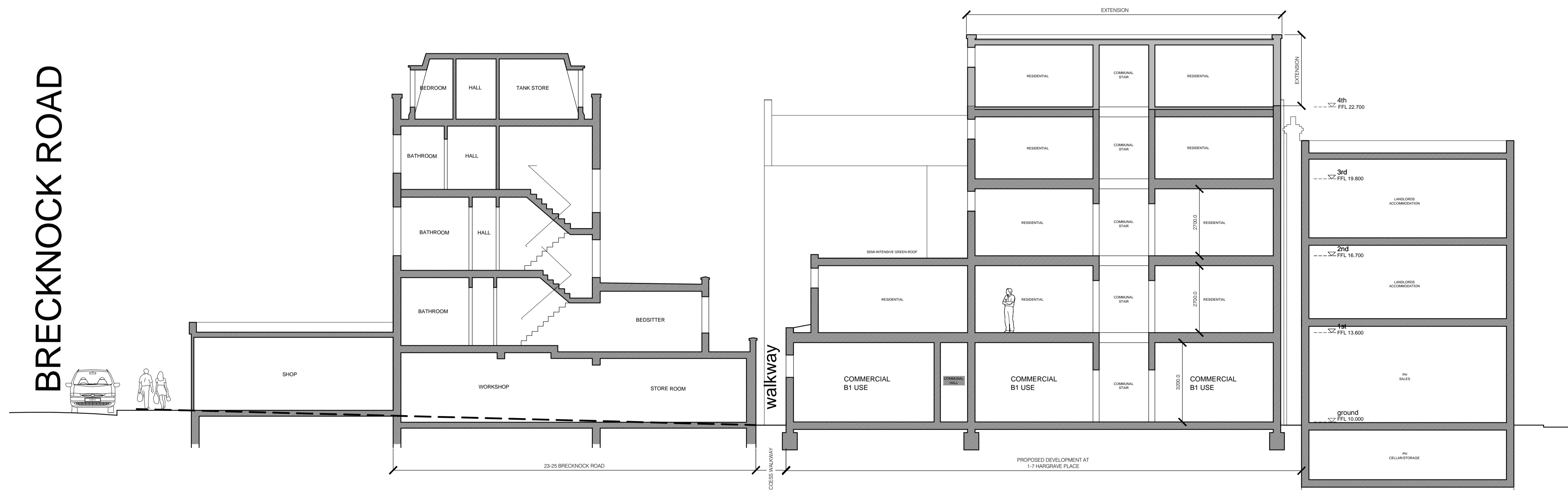
SITE SECTION B-B 1:100 @ A1
