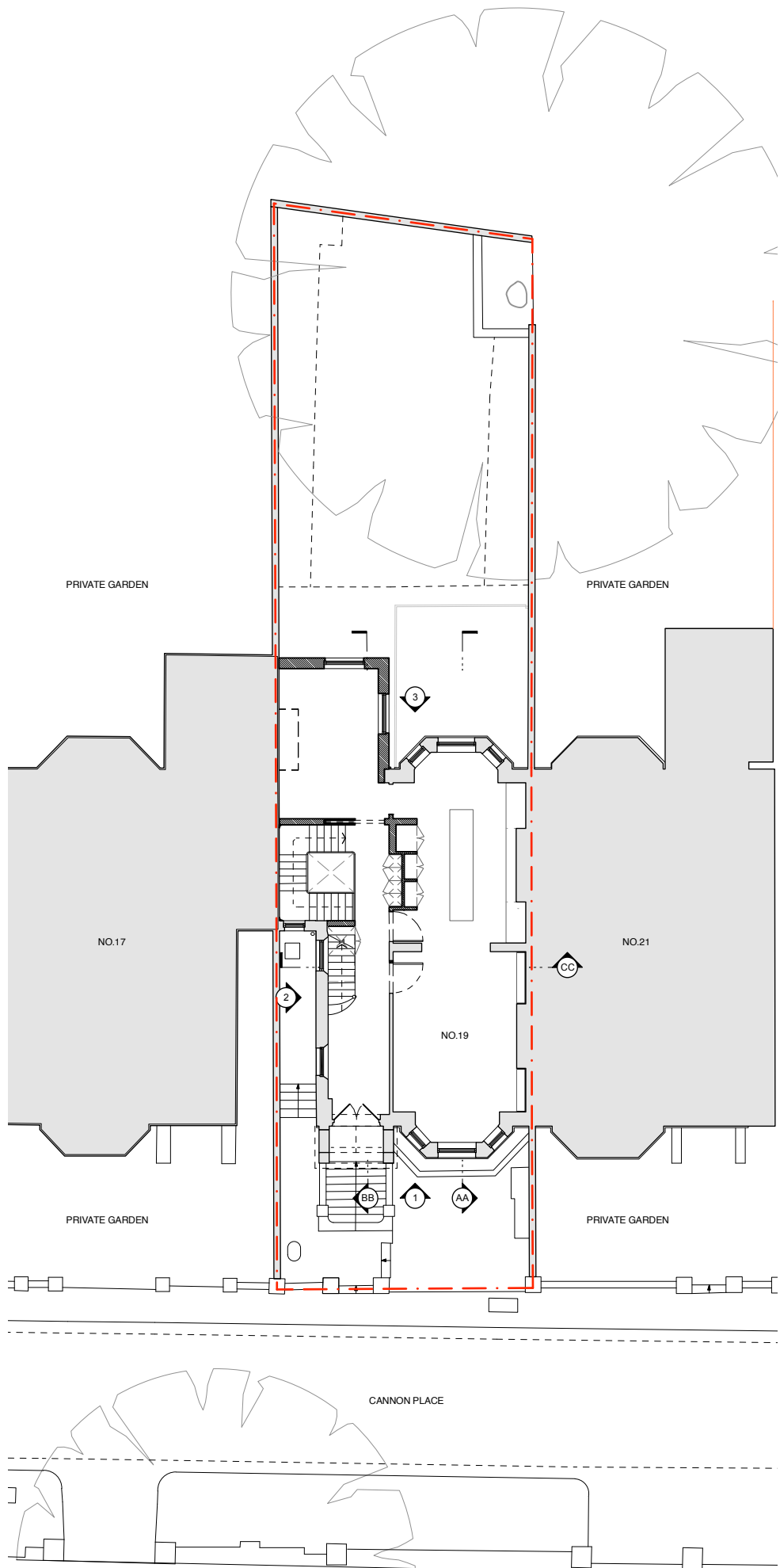
1 Proposed Site Plan Scale: 1:200
