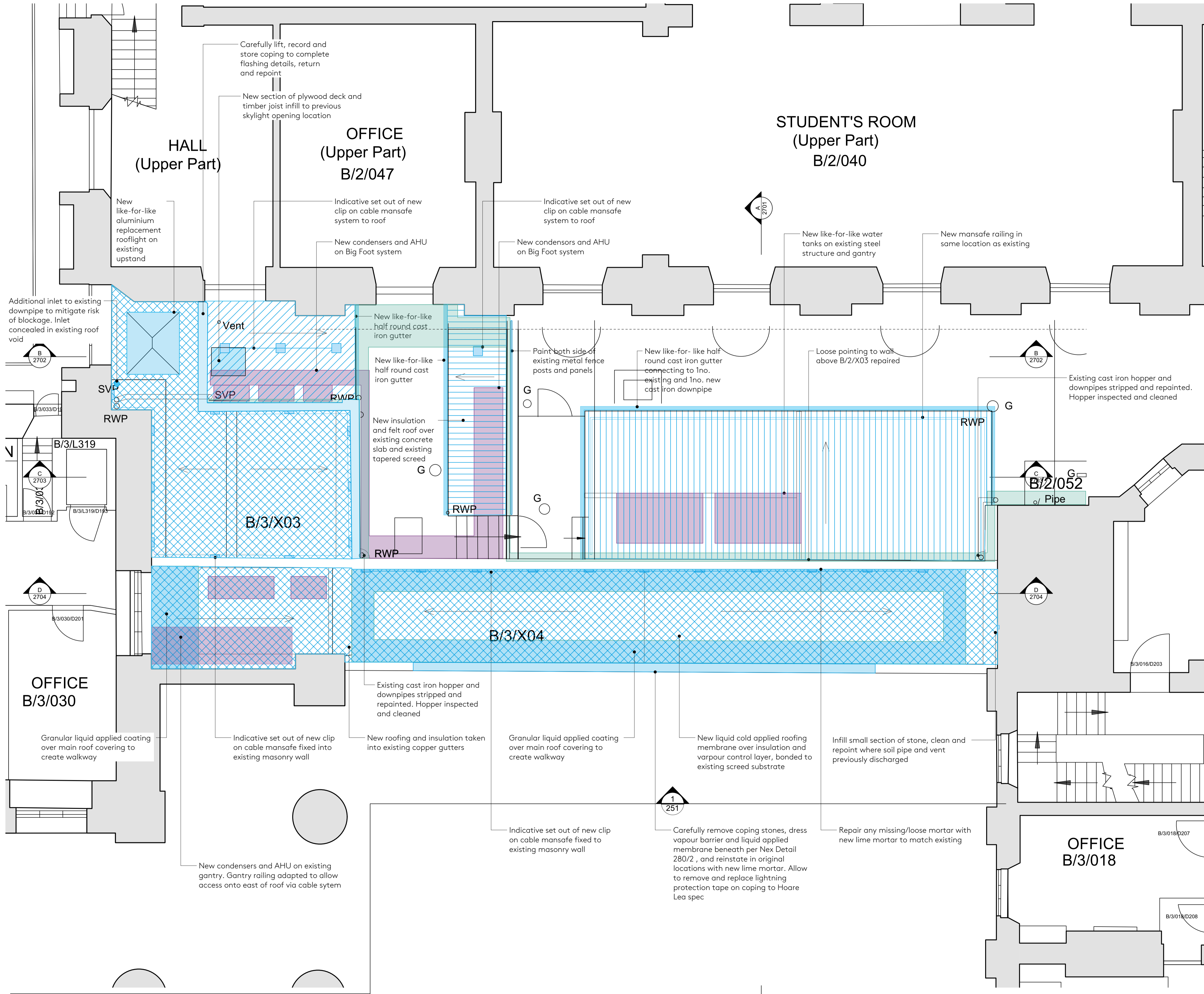
1 Roof Plan - Proposed Scale: 1:50
