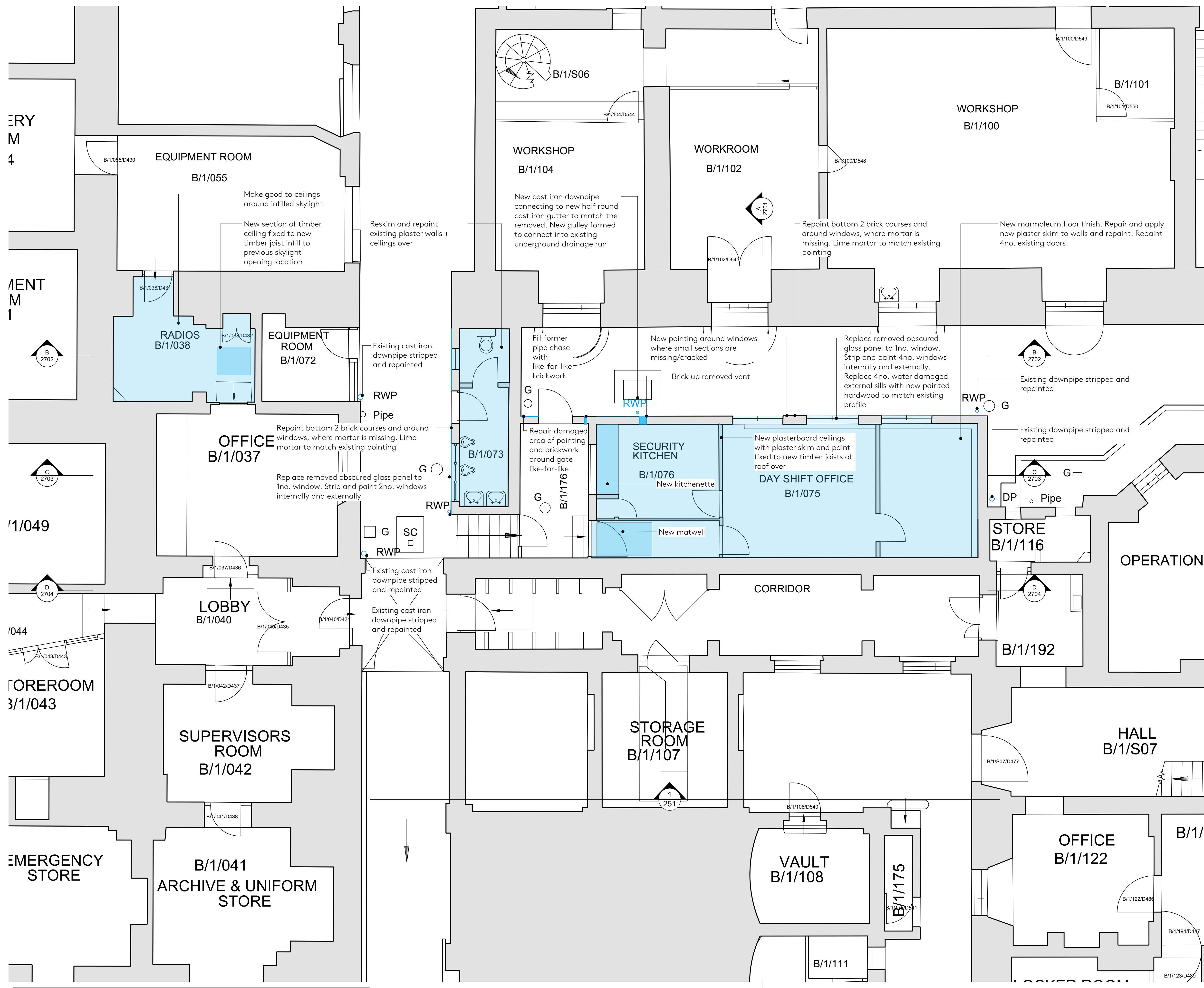
1 Basement Floor Plan - Proposed Scale: 1:50
