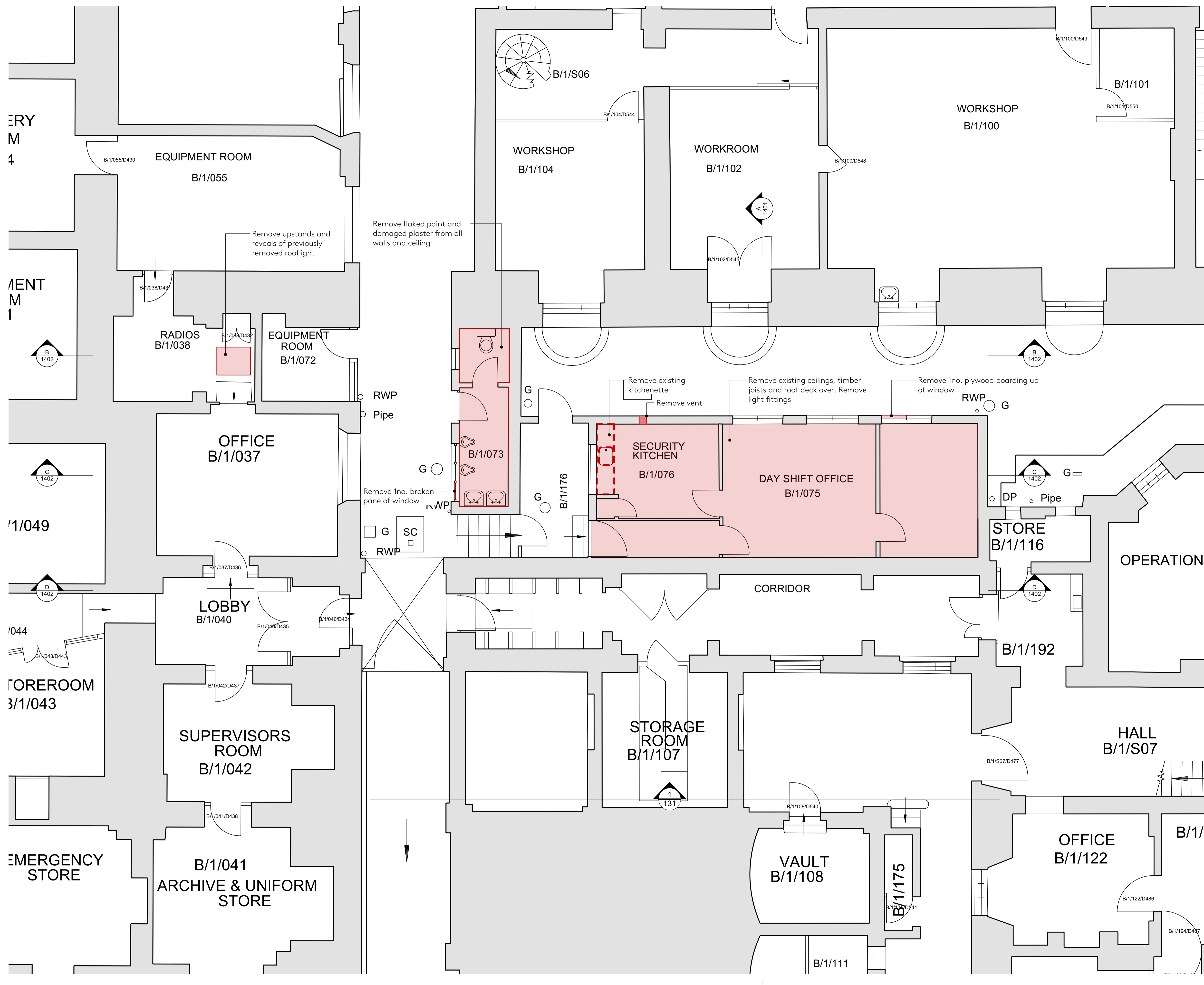
1 Basement Floor Plan - Existing Scale: 1:50
