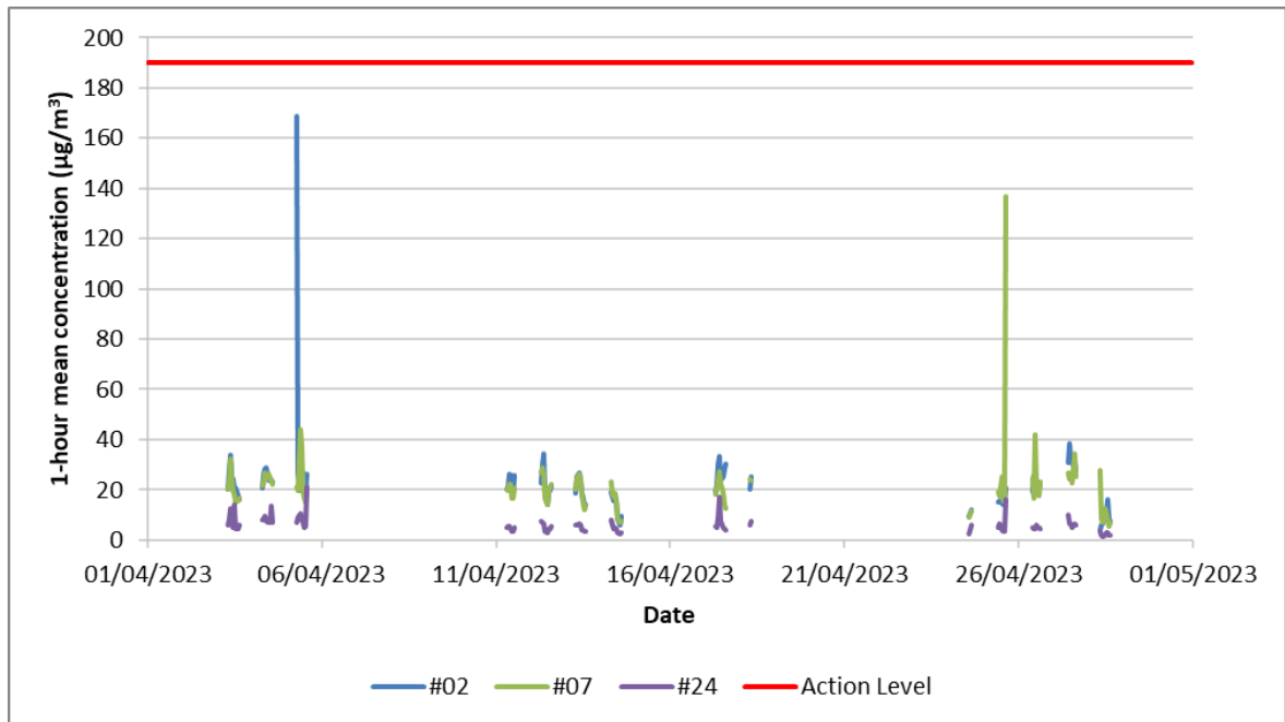
Figure 5: Measured 1-Hour Mean PM 10 concentrations at Monitors #02, #07 and #24 during April 2023
