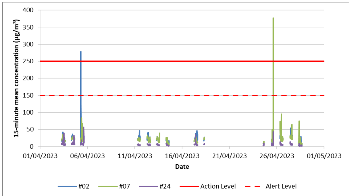
Figure 6: Measured 15-Minute Mean PM 10 concentrations at Monitors #02, #07 and #24 during April 2023
