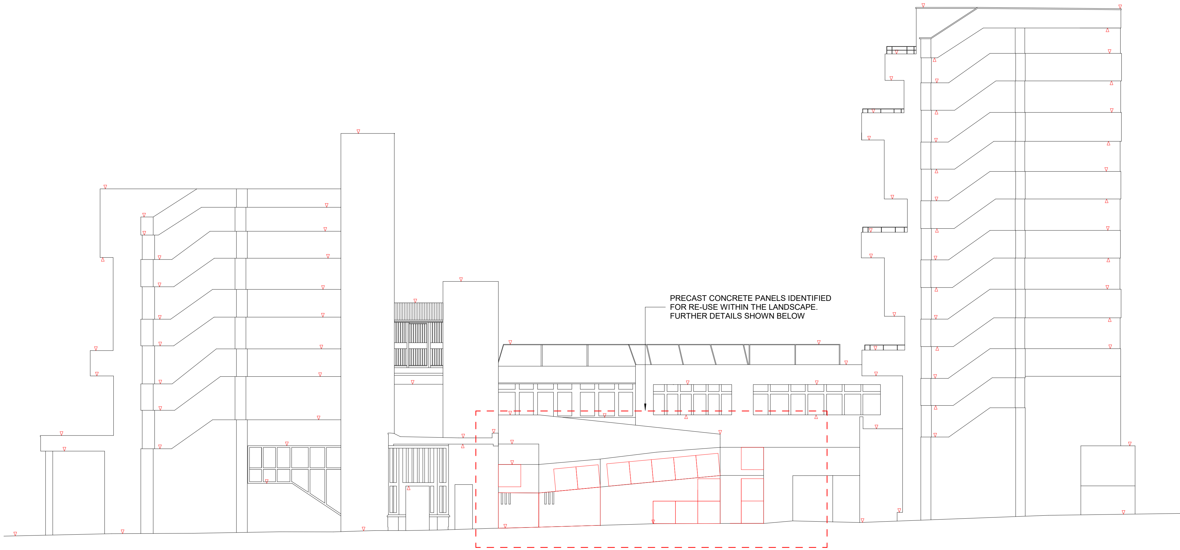
1 ELEVATION - Hinstock Facade 1 : 100
