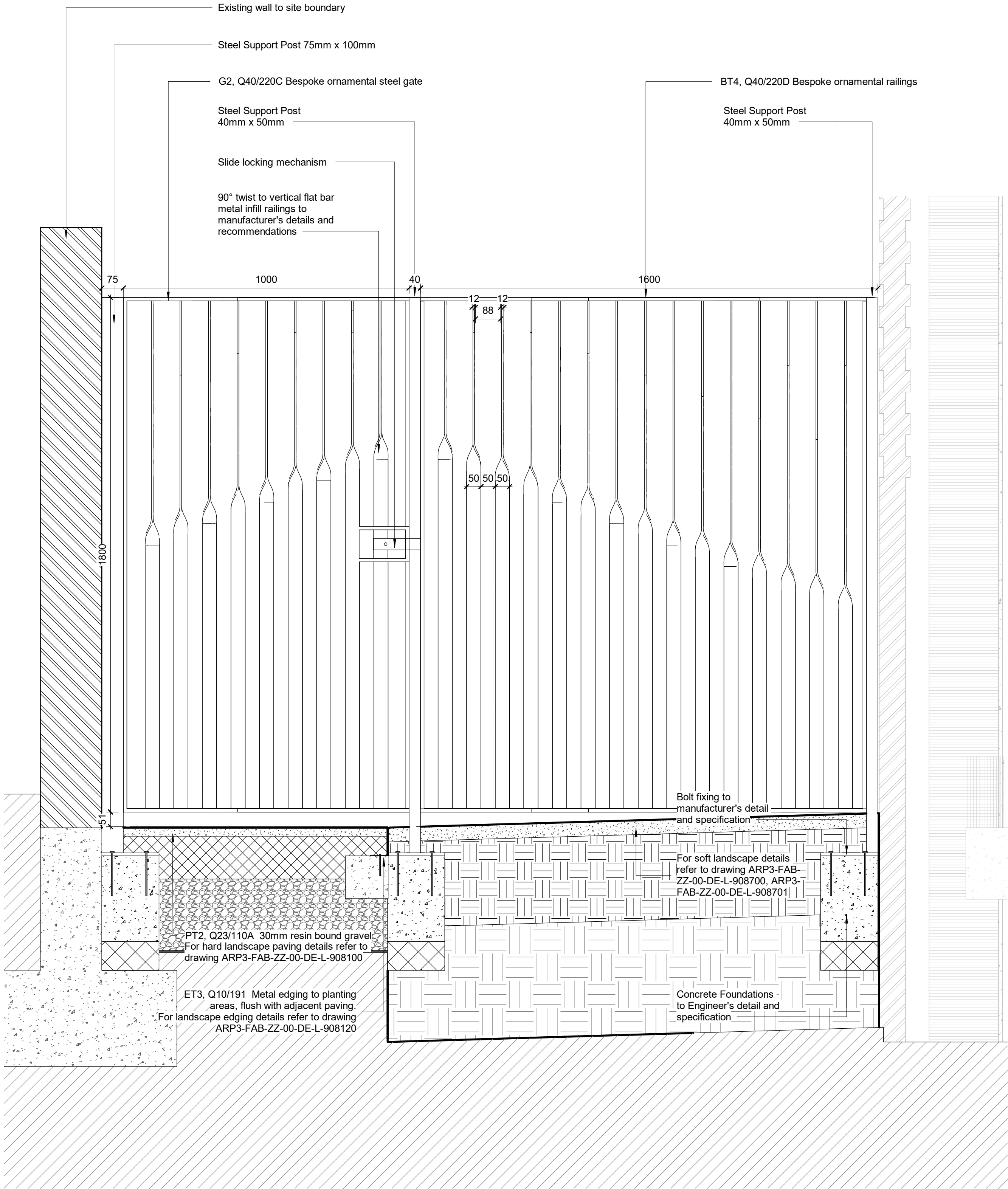
1 BT4 Ornamental Railing and G2 Ornametal Gate Details 1 : 10
