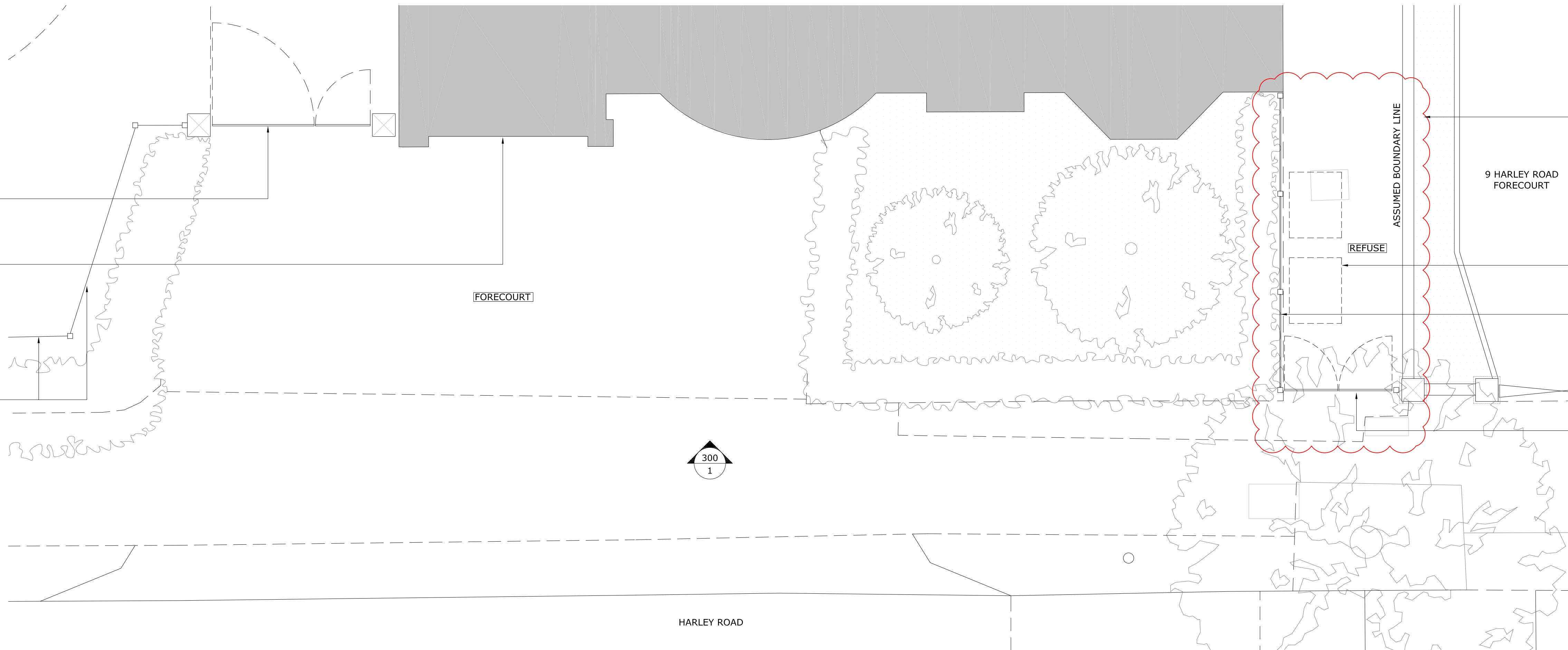
3 PROPOSED FORECOURT PLAN 1:50@A1, 1:100@A3
