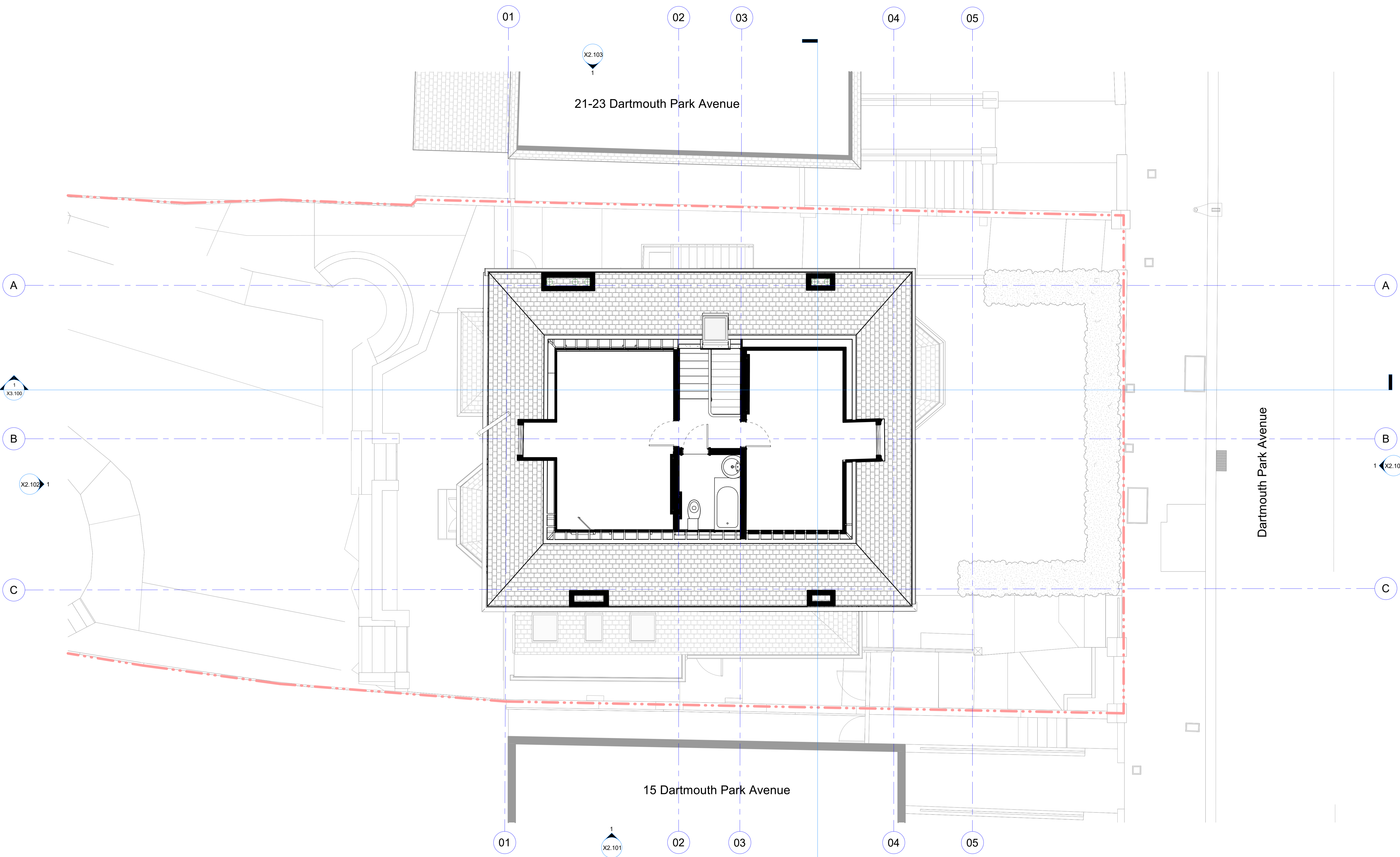
1 Second Floor Plan - Existing 1 : 50
