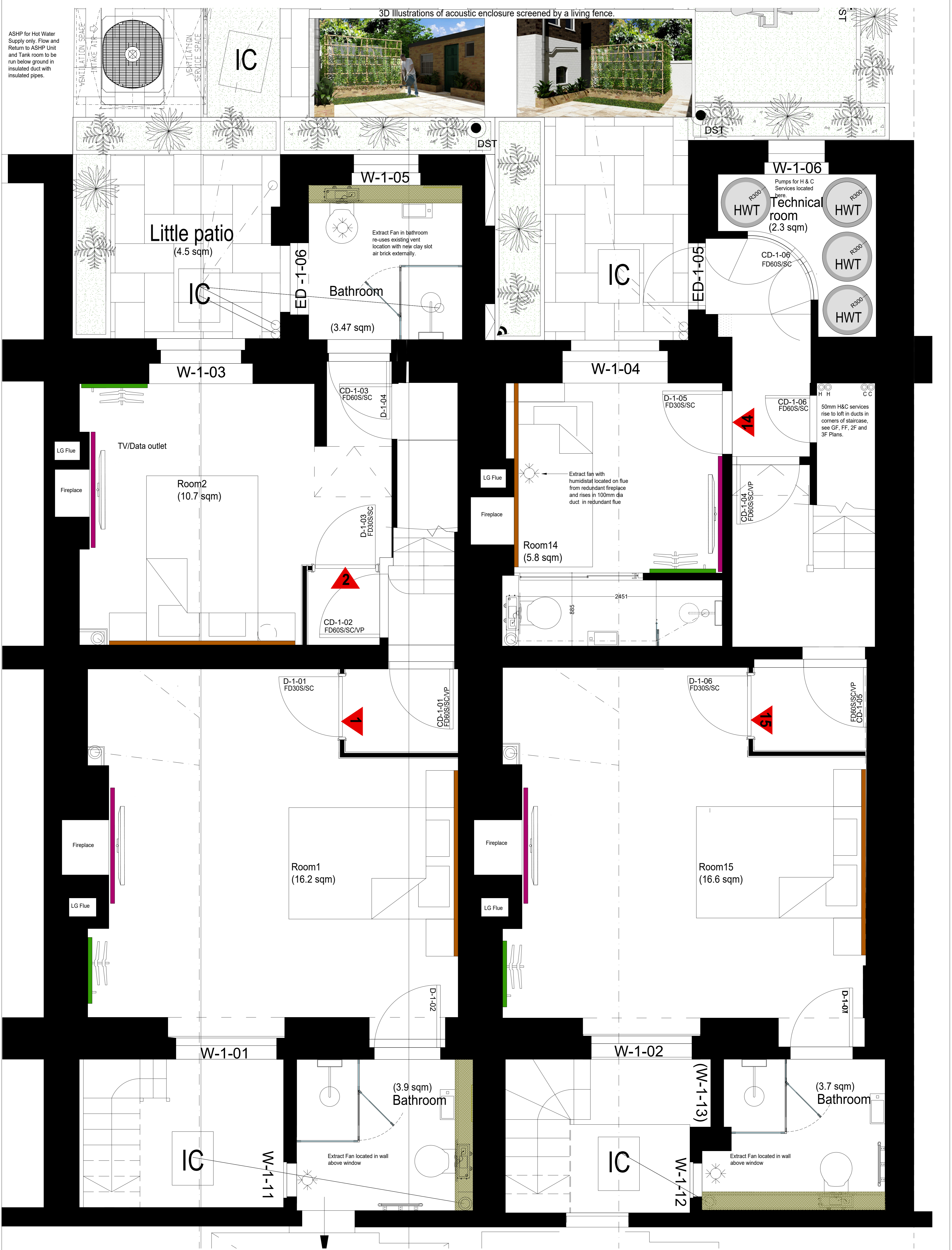
Proposed Lower Ground Floor Plan
