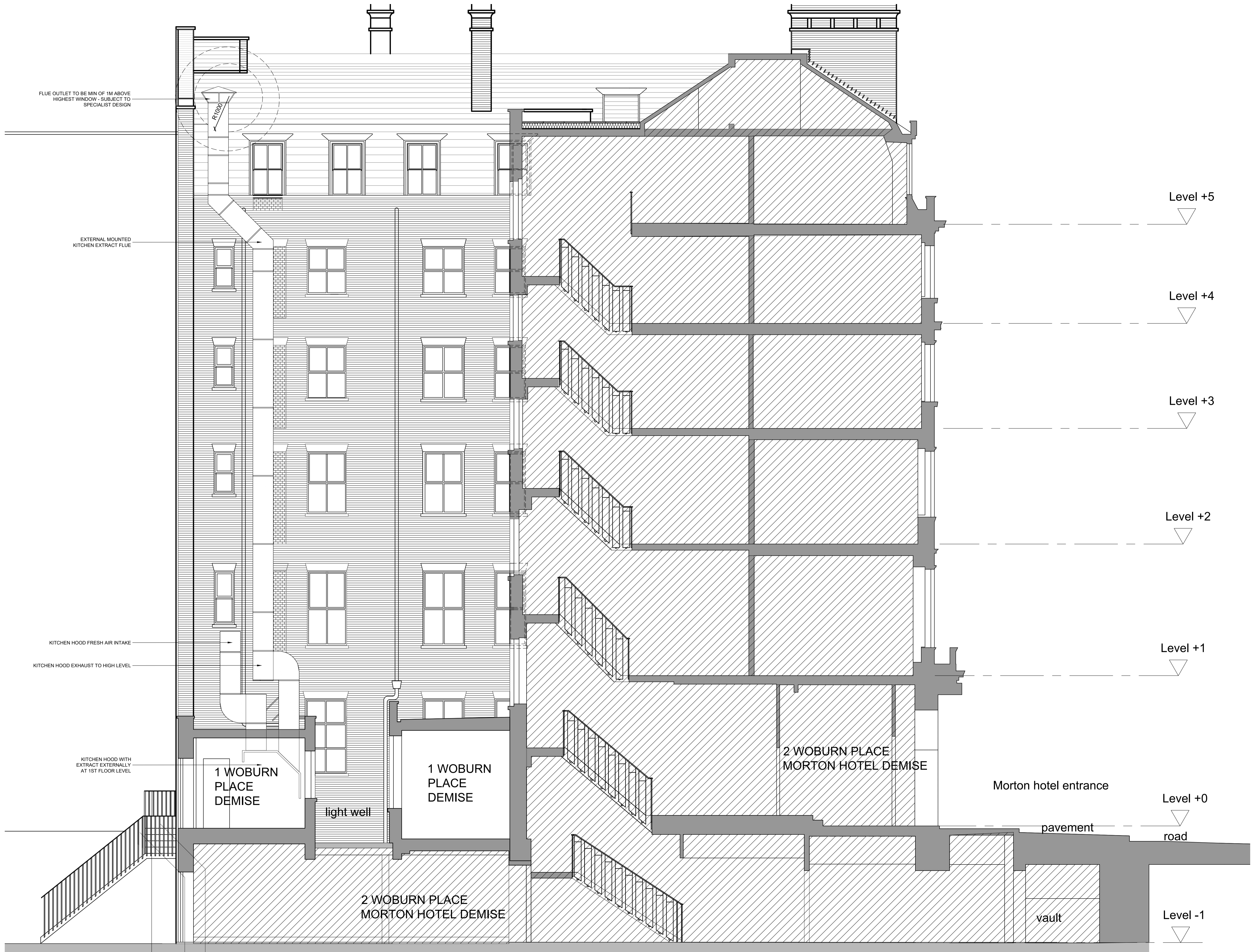
1 SECTION - AA -
