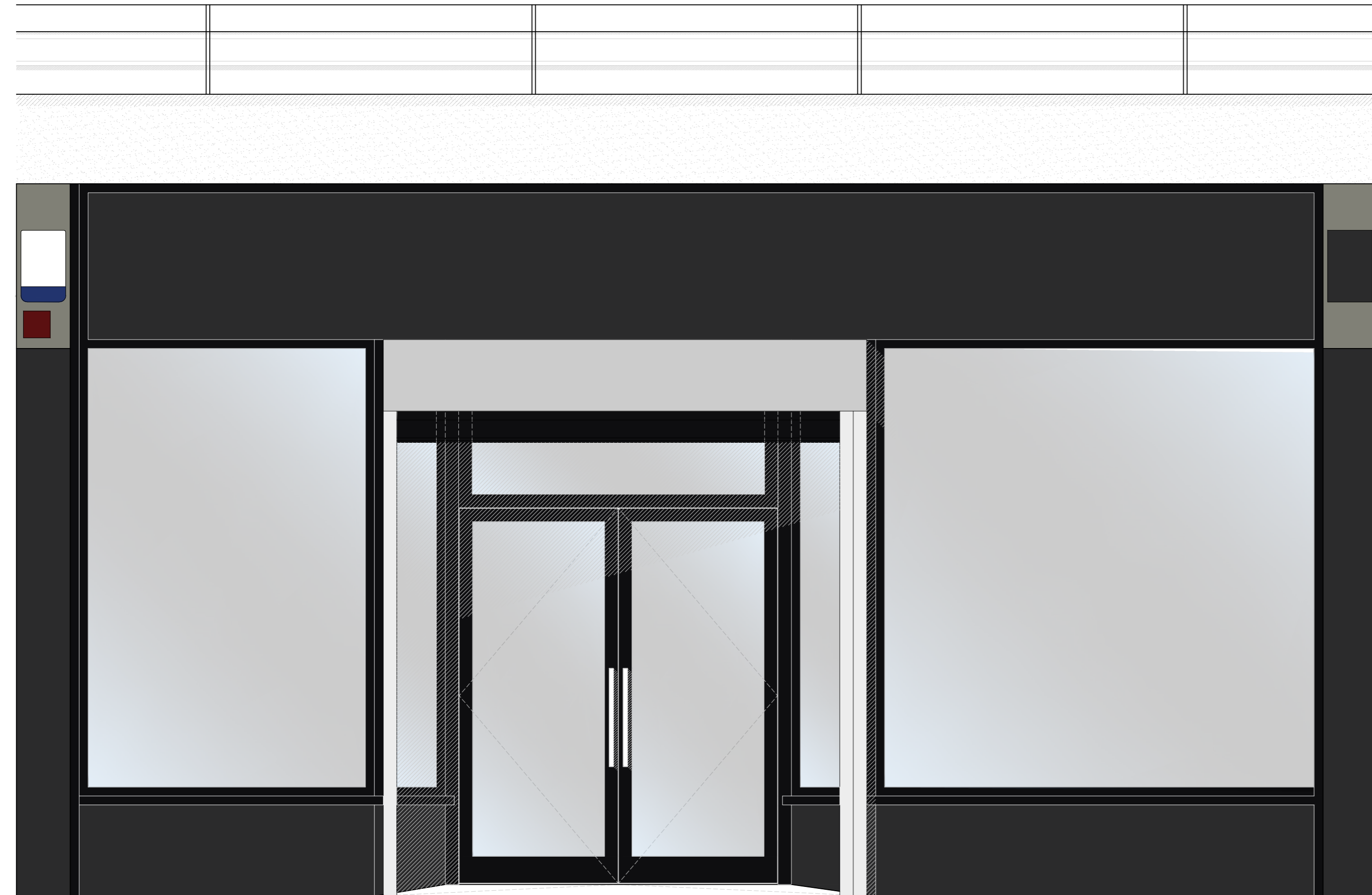
1 PROPOSED SHOP-FRONT ELEVATION (FRONT) 1:20 @ A2
