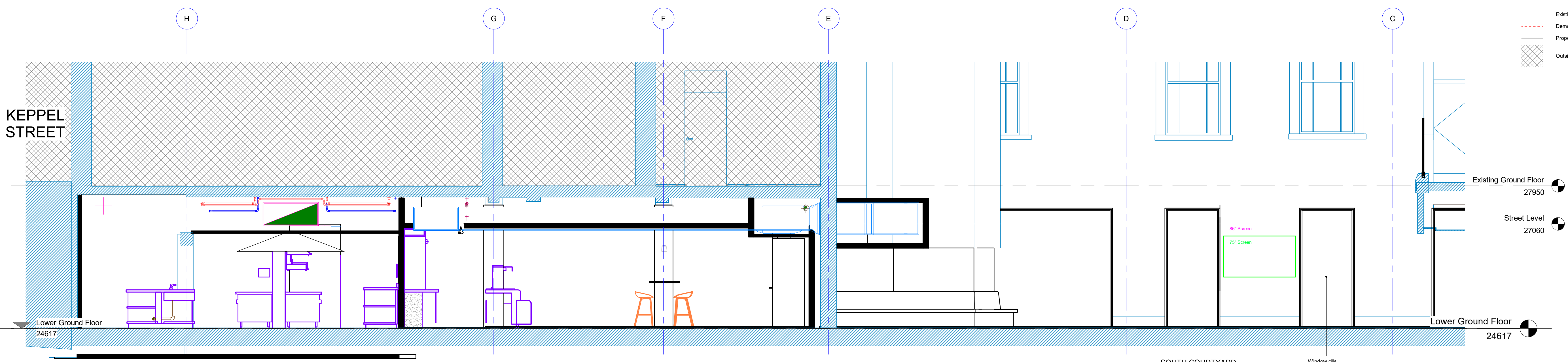
1 Proposed - Section AA 1 : 50
