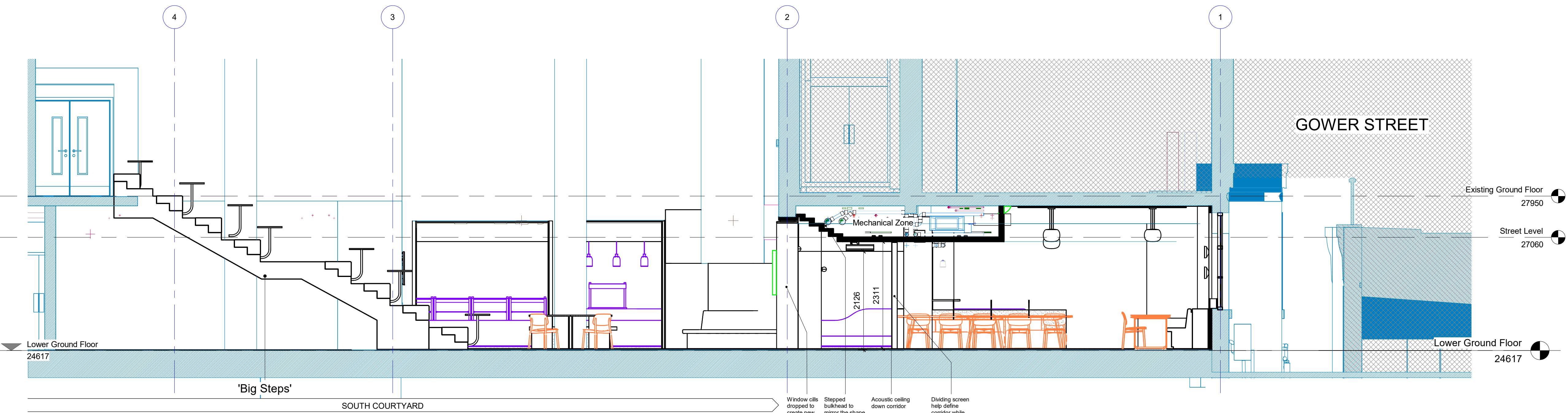
2 Proposed - Section BB 1 : 50
