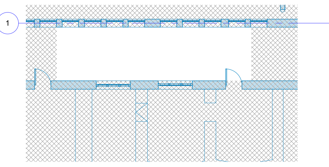
2 Demo - LG Gower Street Escape Stair RCP 1:100
