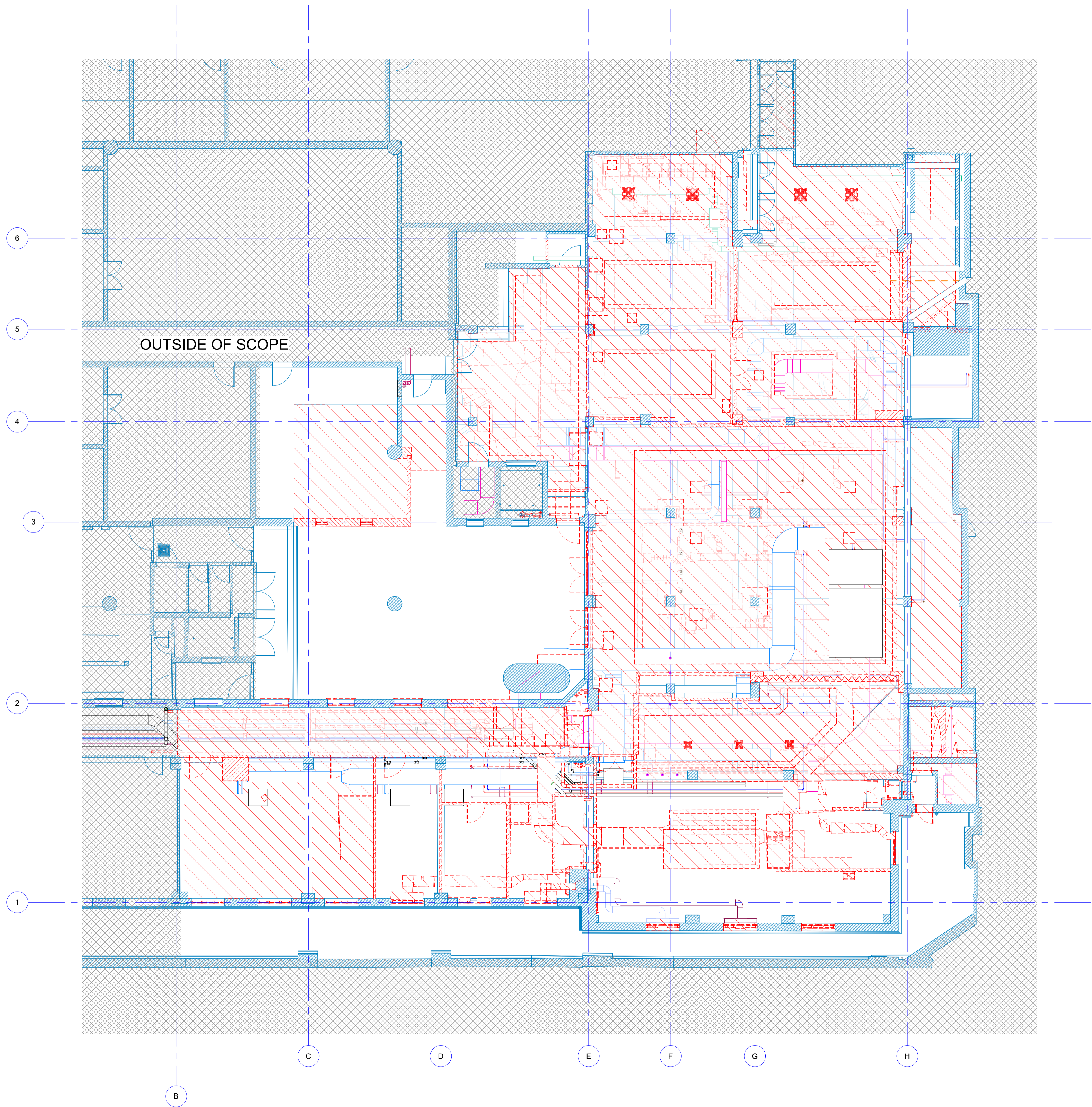
1 Demo RCP - Lower Ground 1:100
