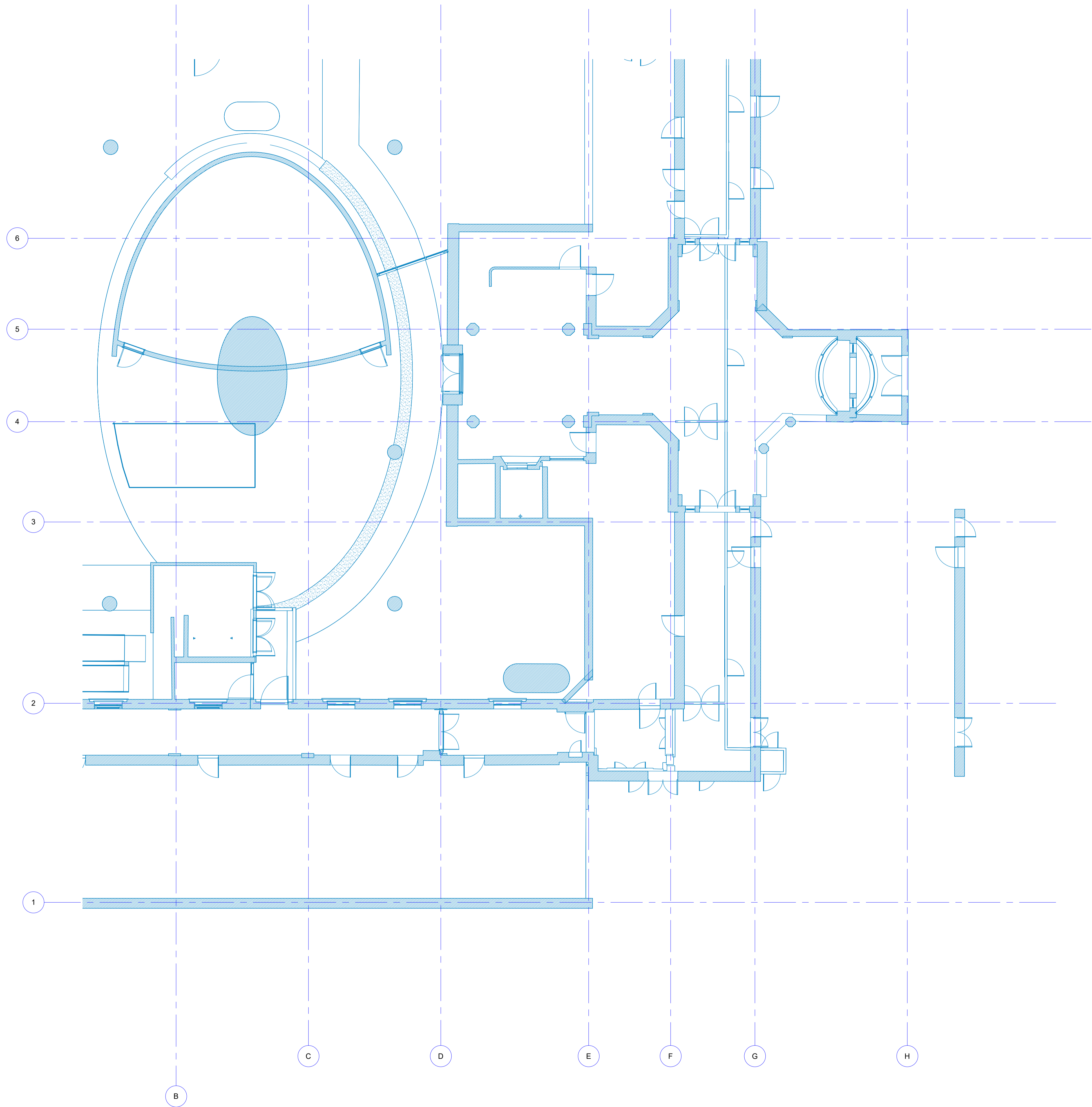
1 Ex RCP - Ground Floor 1:100
