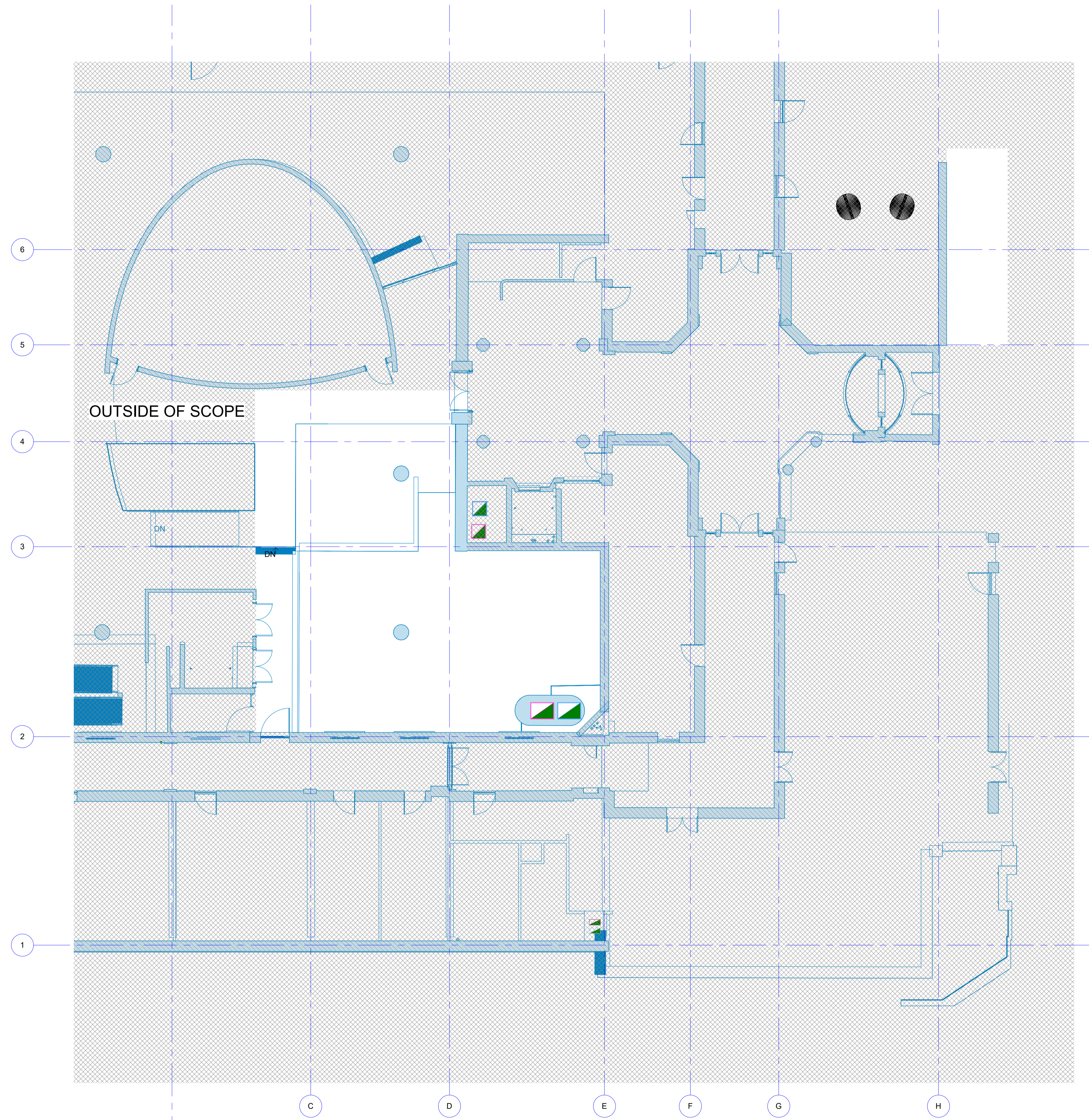
1 Ex. GA - Ground Floor 1 : 100
