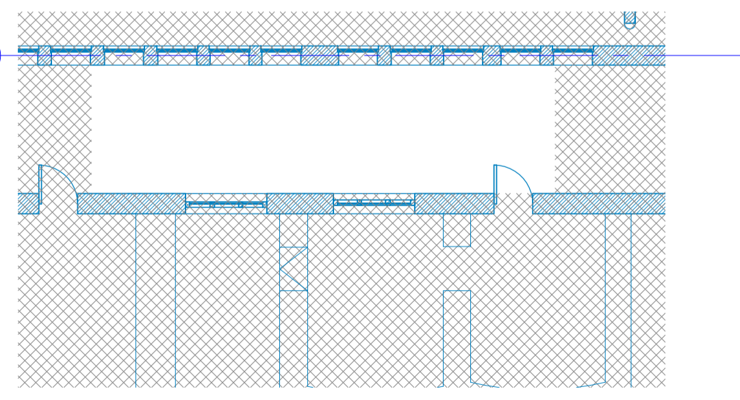
2 Ex. GA - LG Gower Street Escape Stair 1:100
