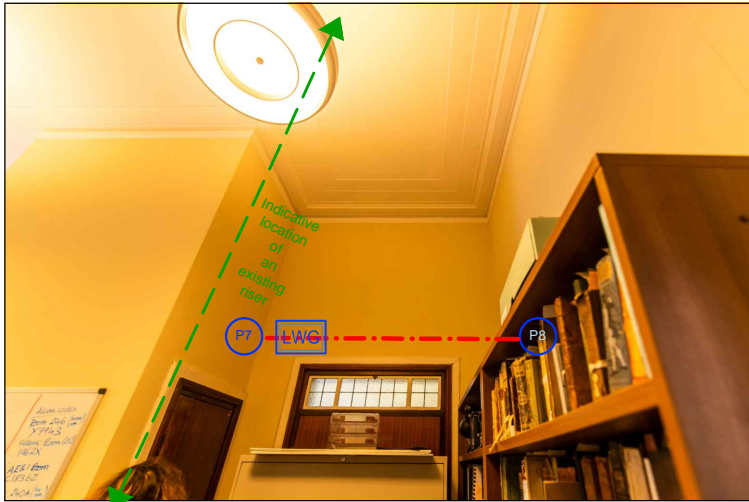
An existing riser in 234A (looking west) and the approximate locations of the proposed conduit and penetrations (subject to specialist contractor). All devices shown are indicative of locations only. Not to scale.
