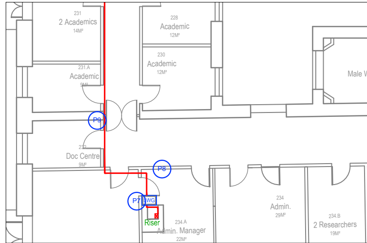
Floorplan showing the devices and associated cabling works to be installed in this location.
