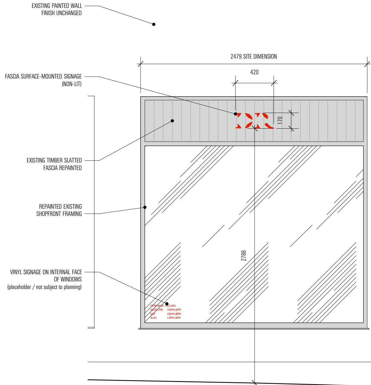
1 PROPOSED - LEFT SIDE ELEVATION PART SCALE: 1:25
