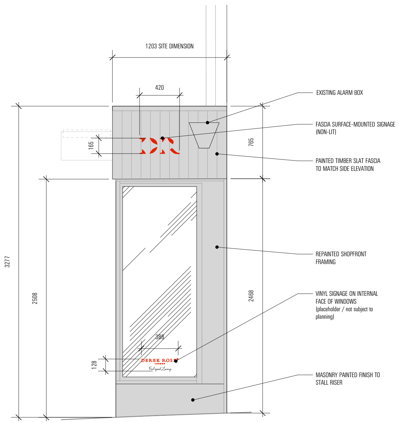
2 PROPOSED - RIGHT SIDE ELEVATION SCALE: 1:25
