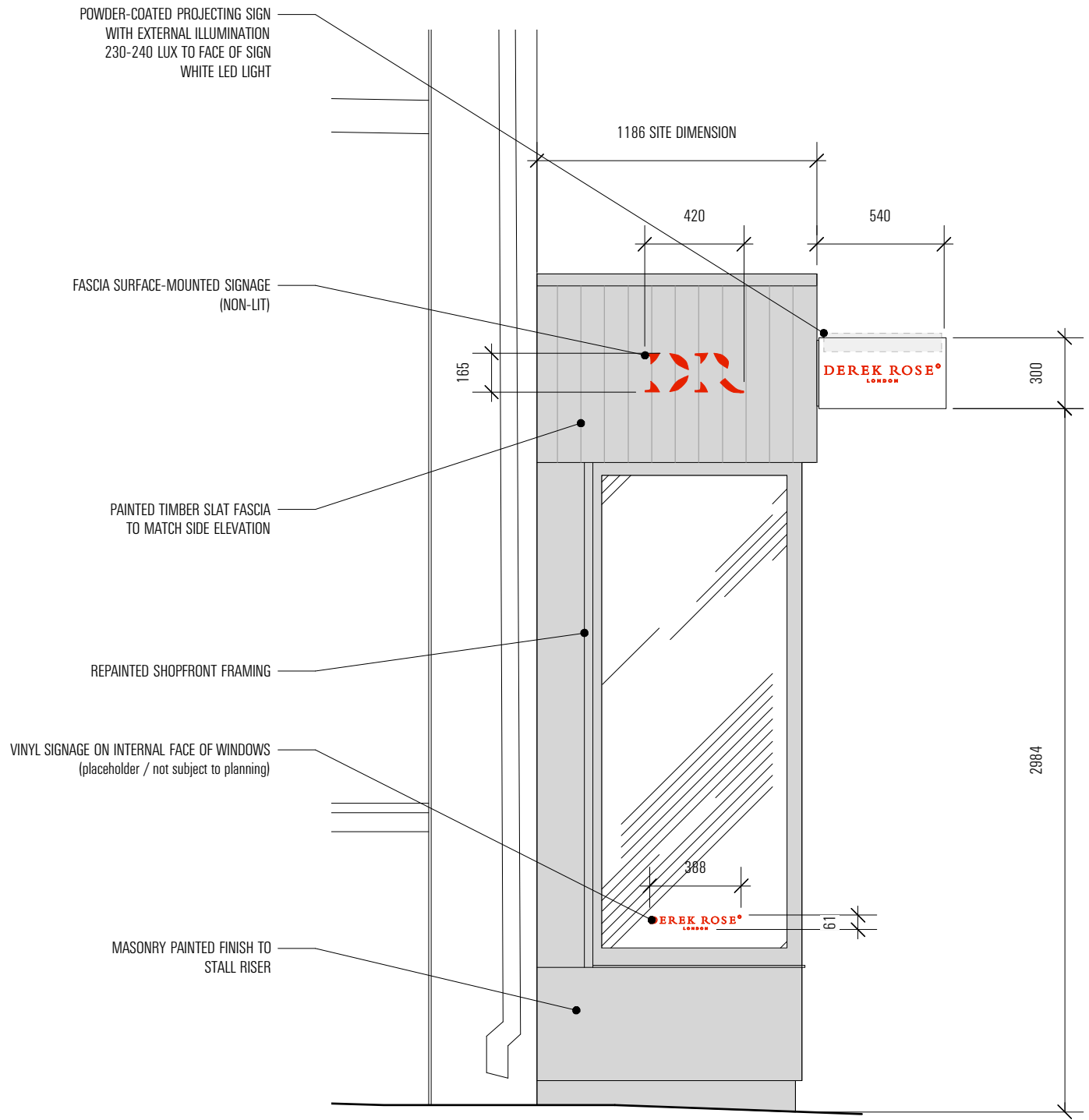
1 PROPOSED - LEFT SIDE ELEVATION PART SCALE: 1:25
