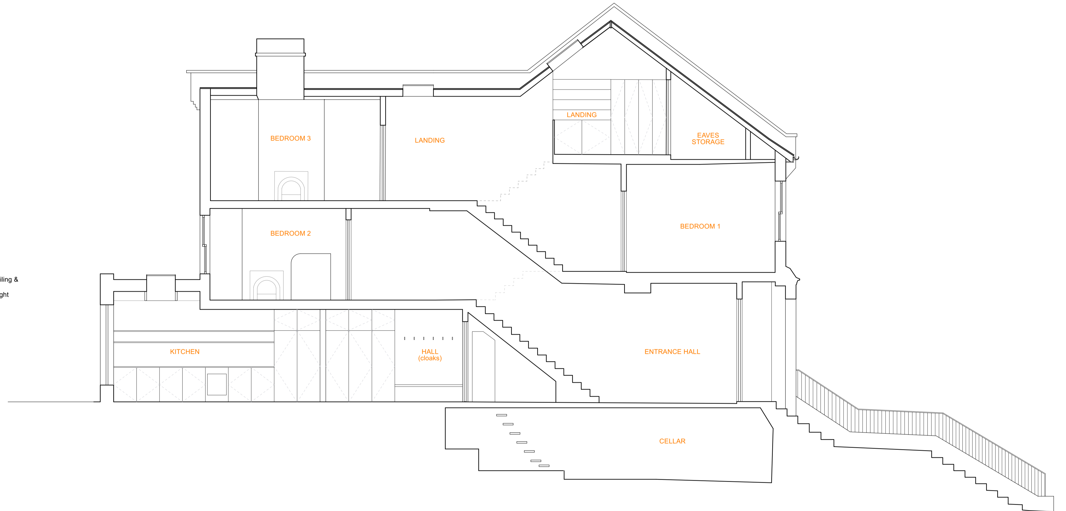
Proposed Section AA
