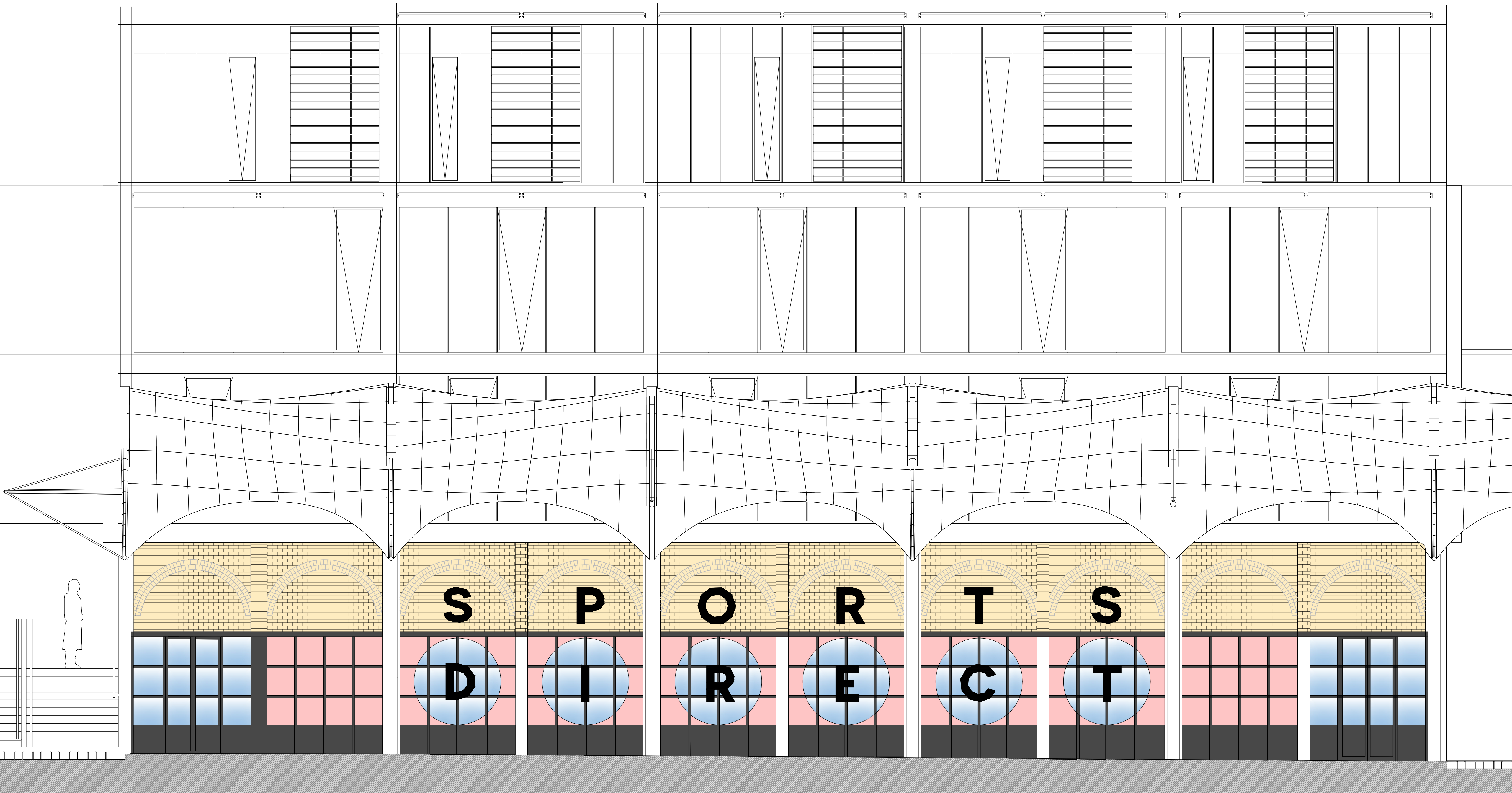
HISTORIC SHOPFRONT / FASCIA SCALE 1:50@A1
