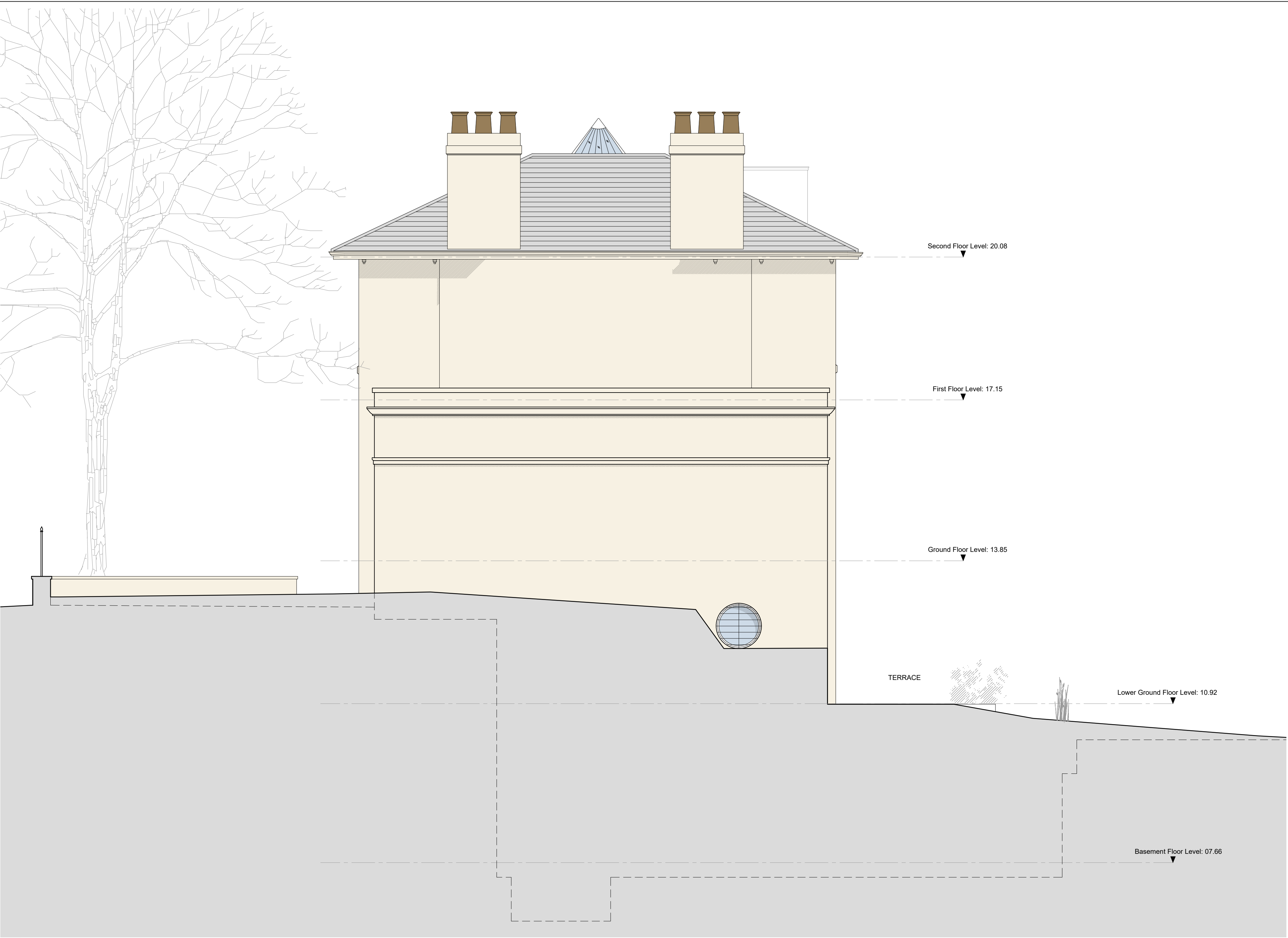
1 Proposed Side (Garage) Elevation 1:50@A2
