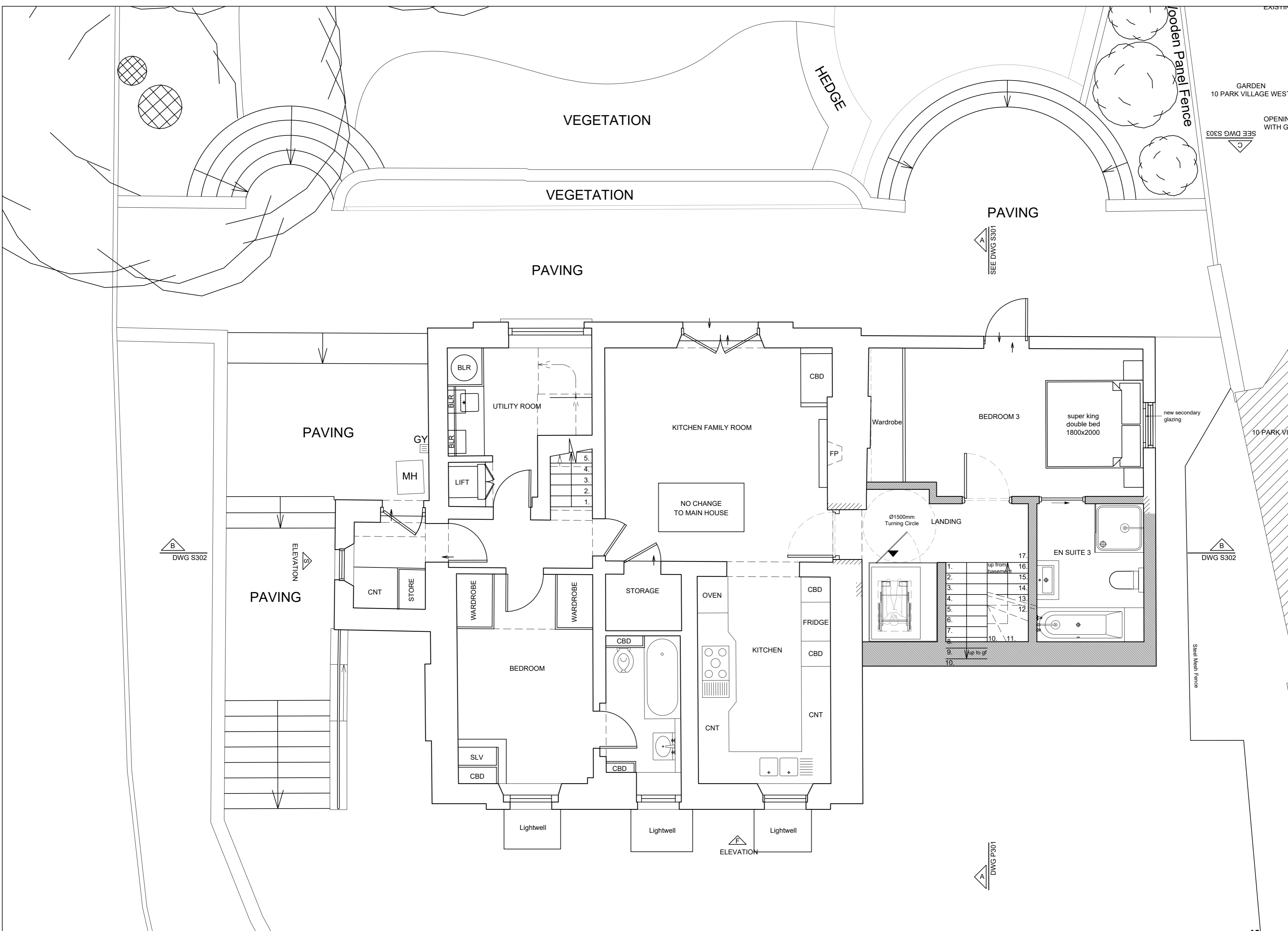
1 Proposed Lower Ground Floor General Arrangement Plan 1:50@A2
