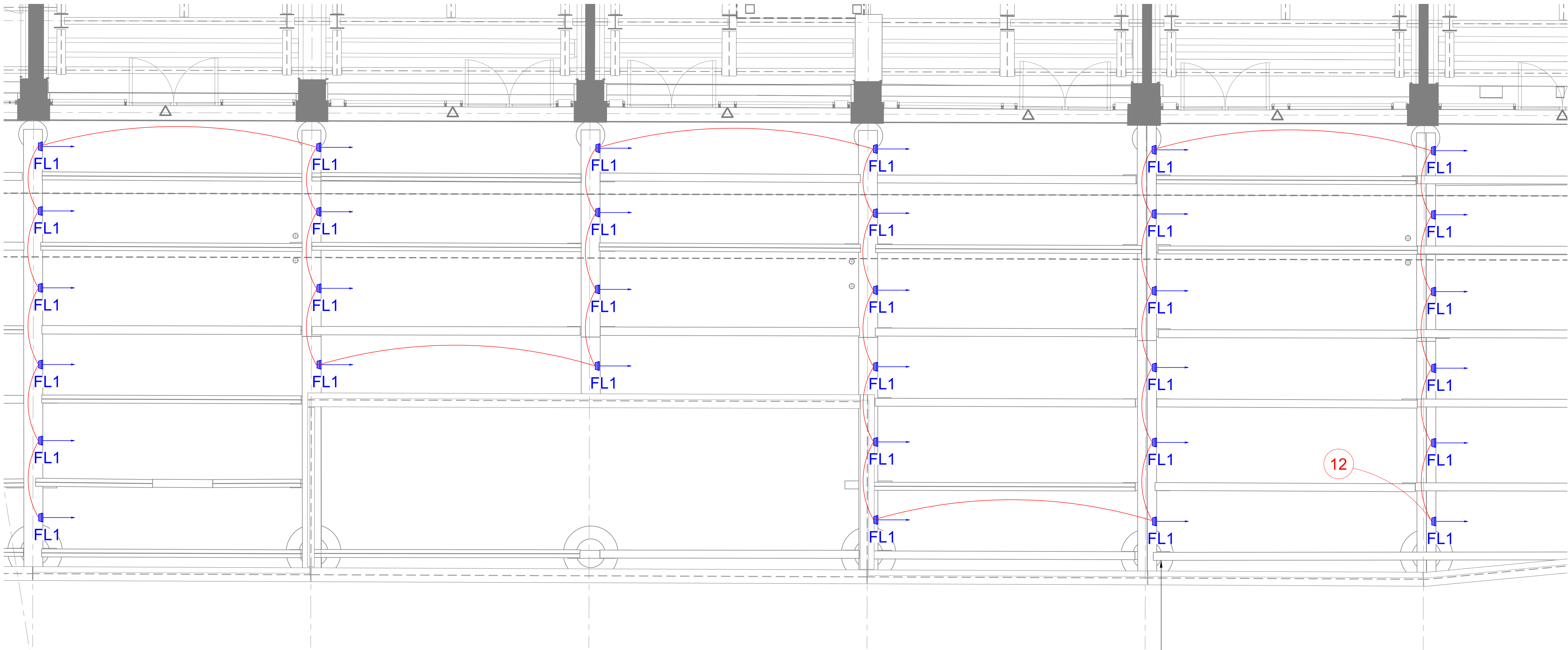
GF VIADUCT LEVEL - 02 Scale 1:50@ A1
