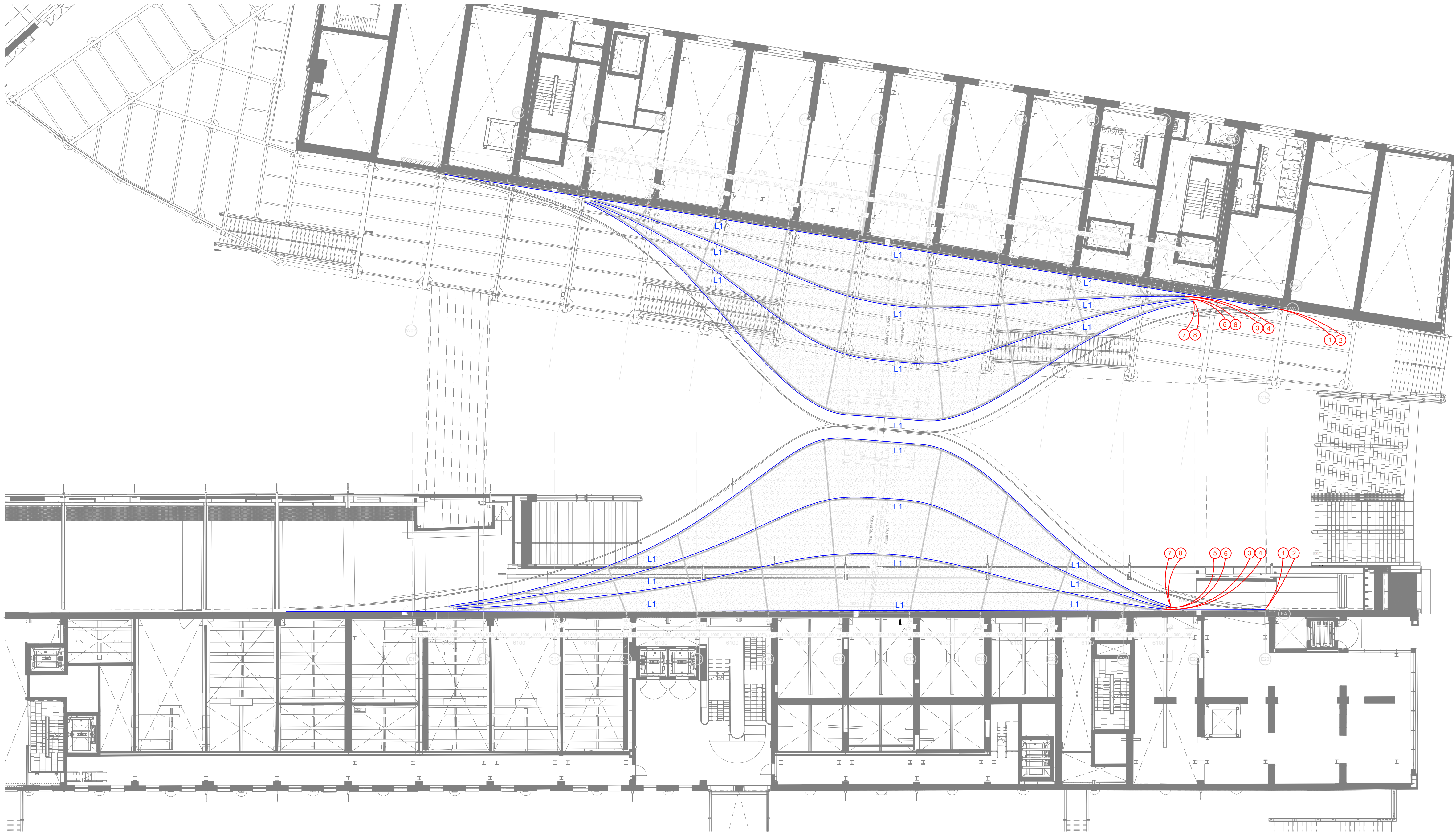
Kissing Roof - Lighting Control Channels Scale 1:200@ A1
