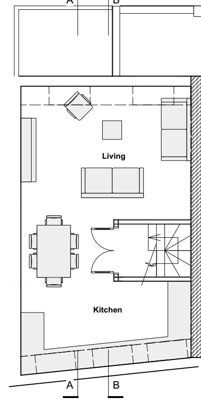
Second Floor Plan as Proposed - 1:100
