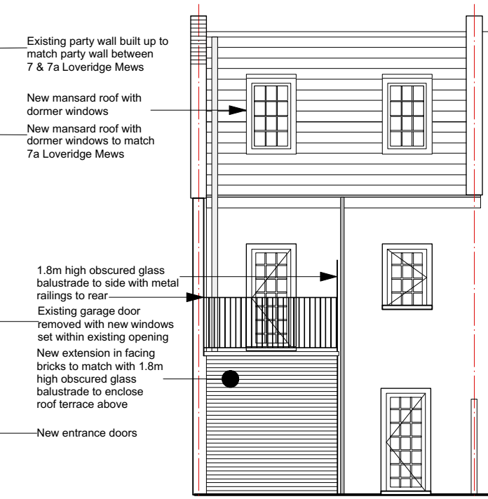
Rear Elevation as Proposed - 1:100
