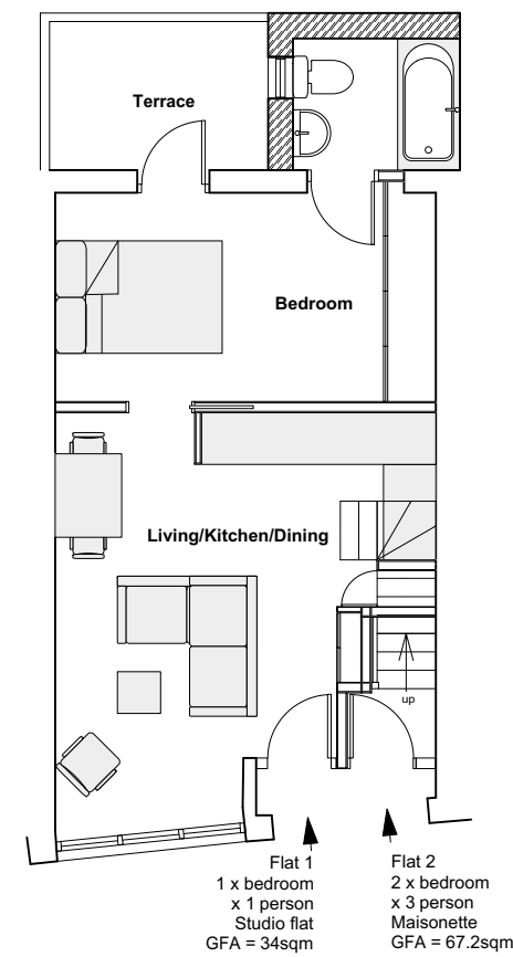
Ground Floor Plan as Proposed - 1:100
