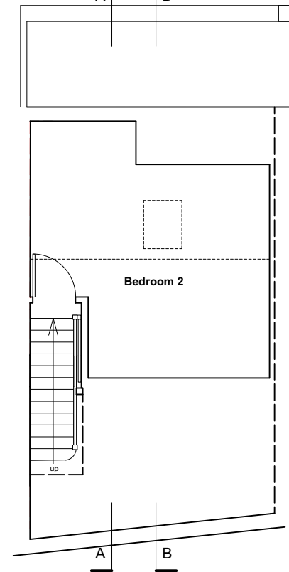
Second Floor Plan as Existing - 1:100
