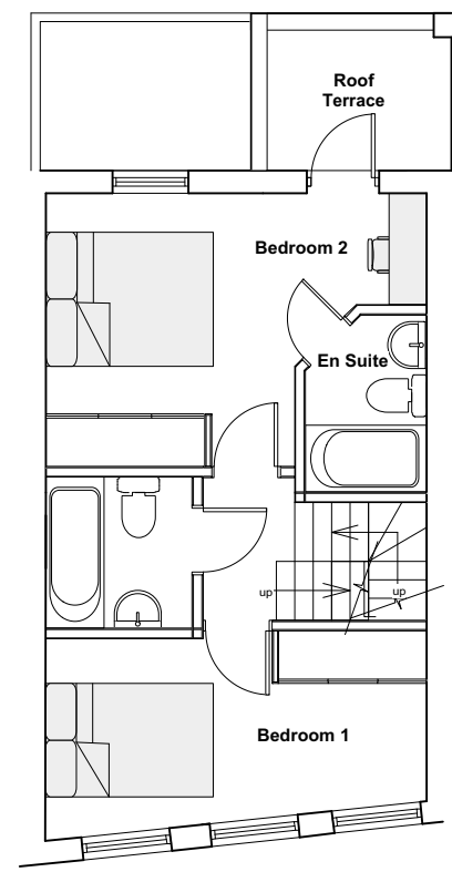
First Floor Plan as Proposed - 1:100
