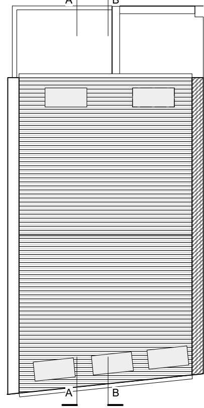
Roof Plan as Proposed - 1:100
