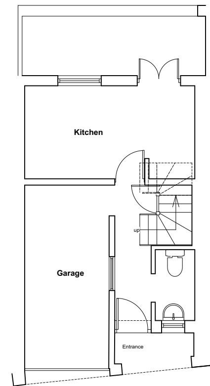
Ground Floor Plan as Existing - 1:100
