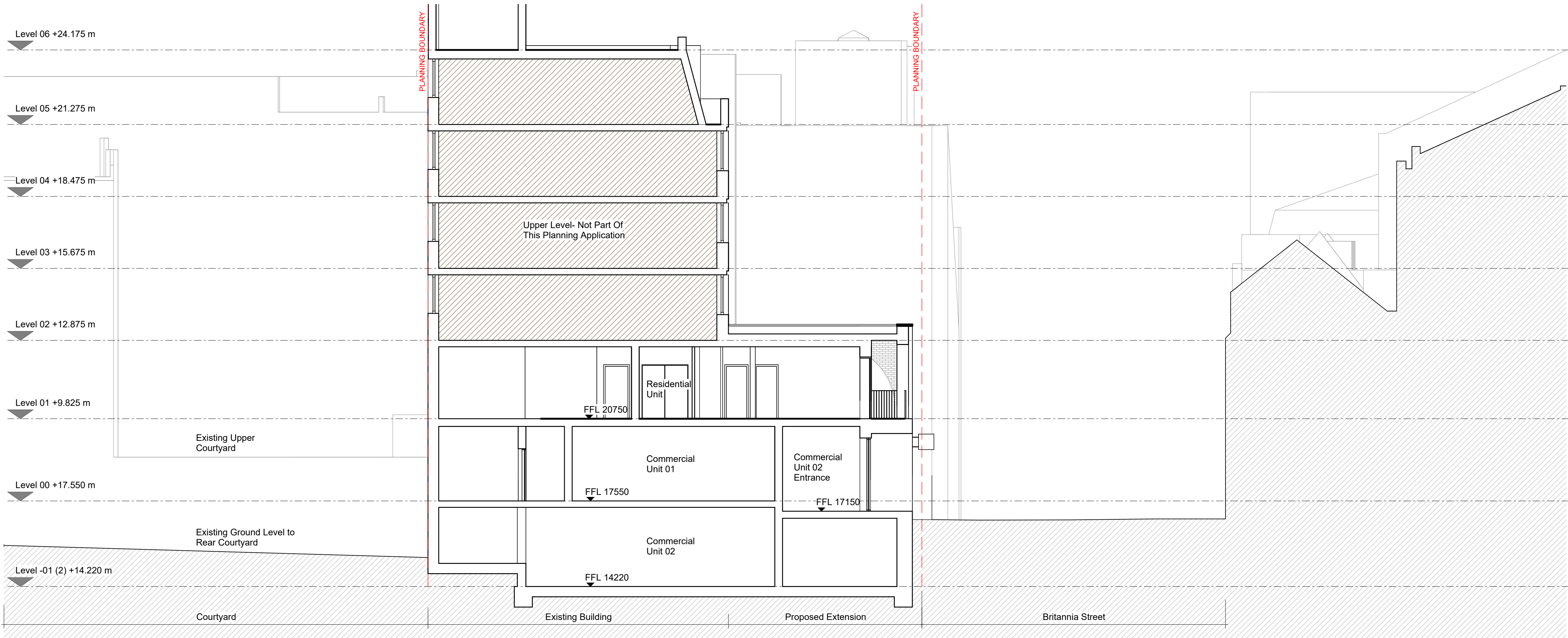
1 Proposed Section AA 1 : 100
