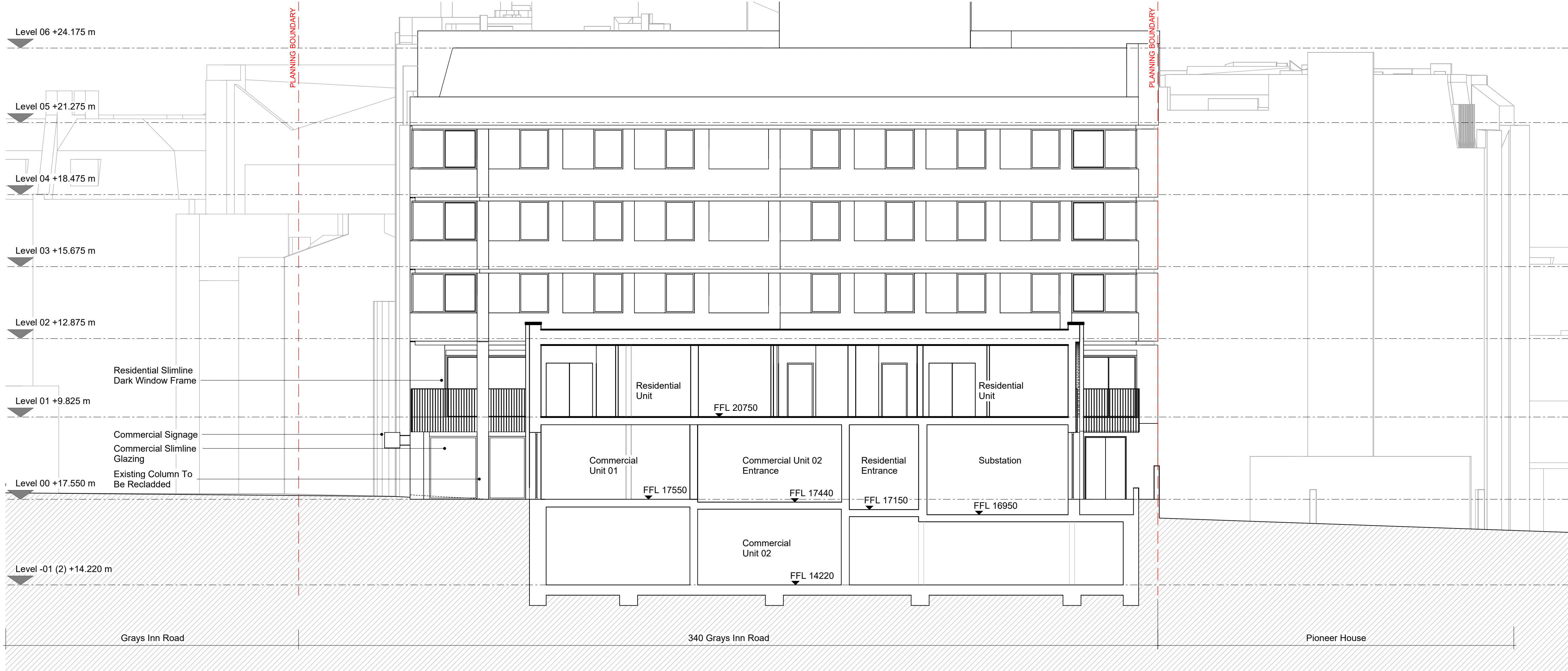
2 Proposed Section BB 1 : 100
