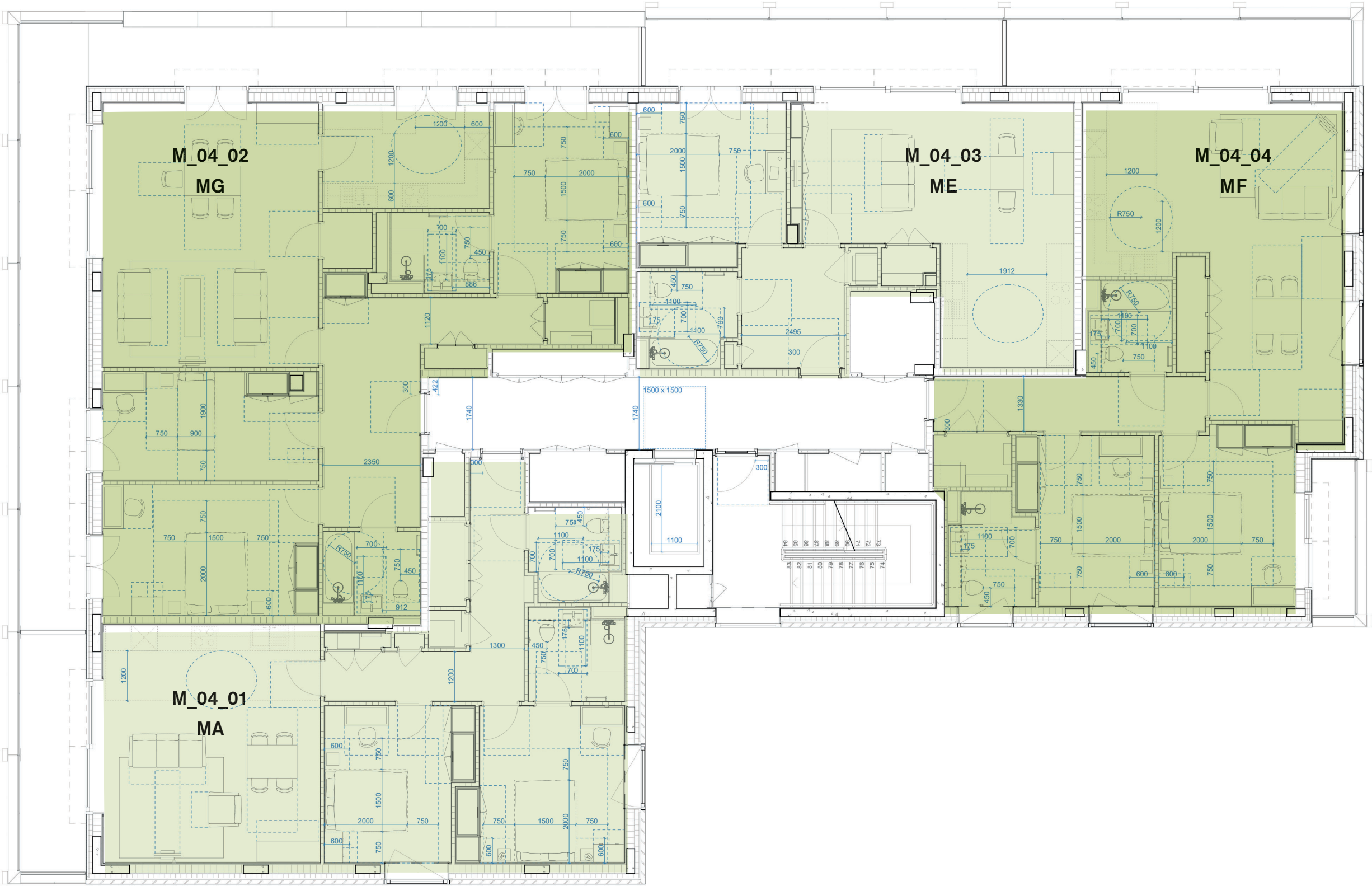
Market building fourth floor plan
