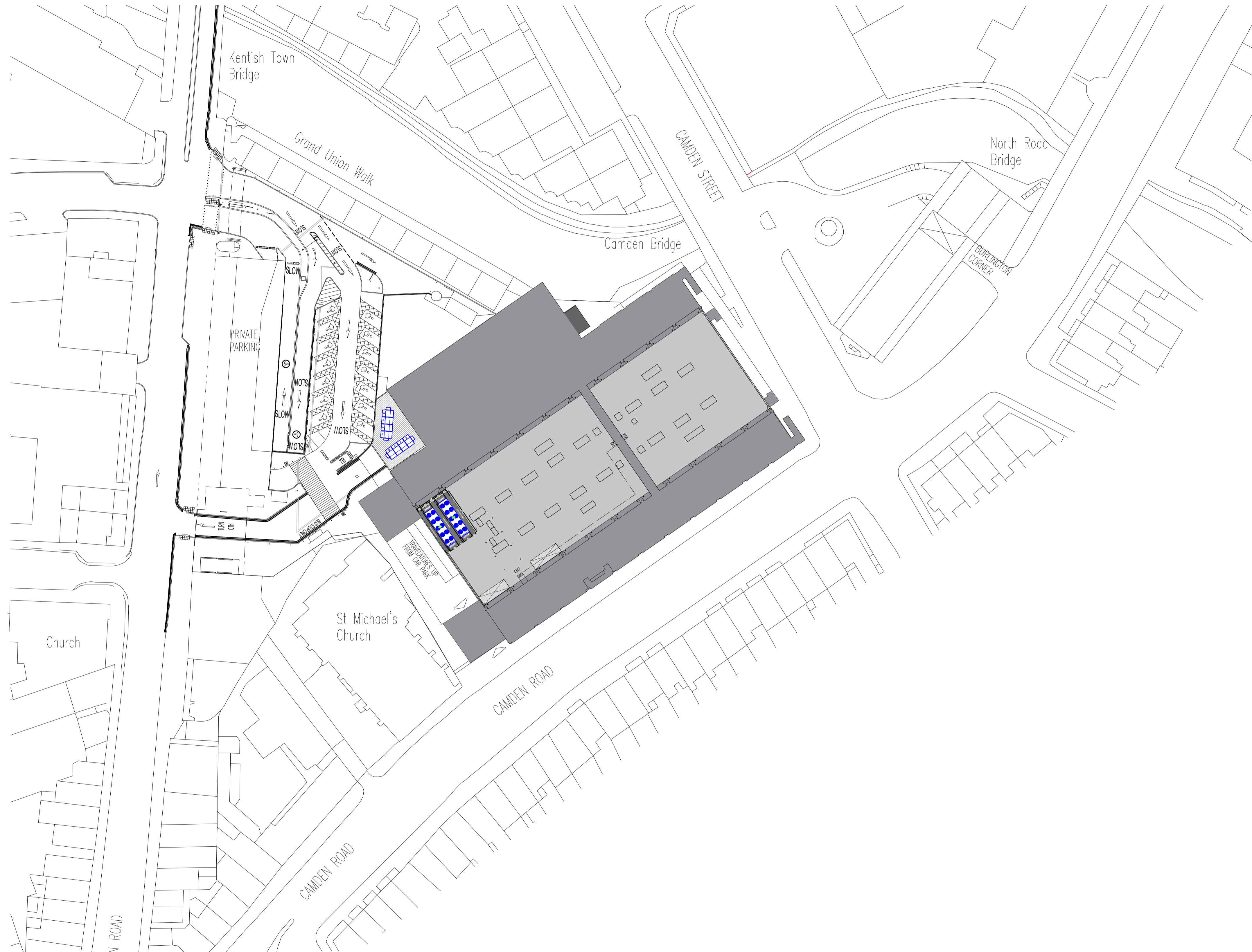
Proposed Site Plan Scale 1:500 @ A1
