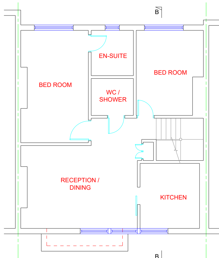
UNCHANGED SECOND FLOOR PLAN
