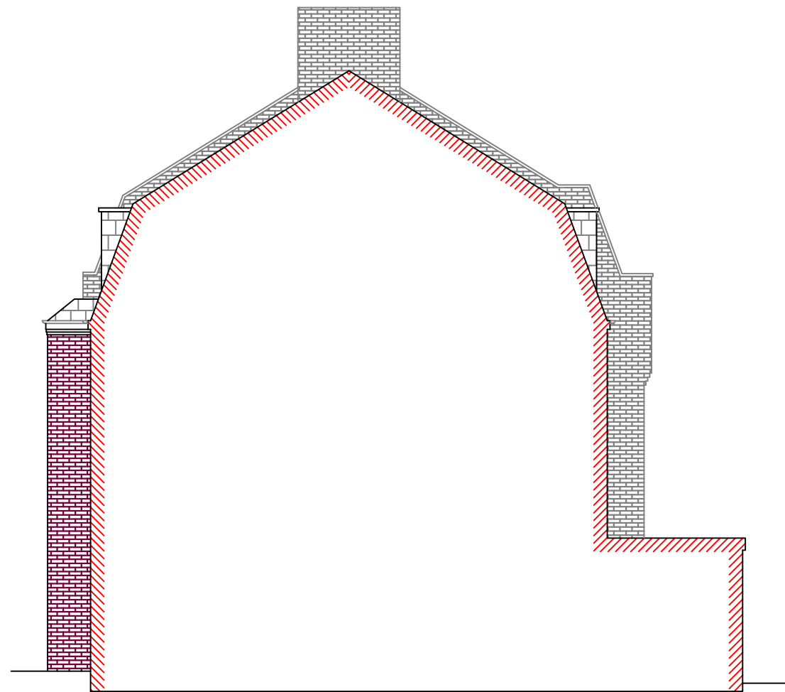
EXISTING RIGHT SIDE ELEVATION
