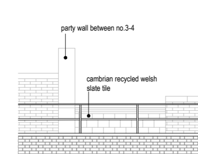
Proposed Elevation DD
