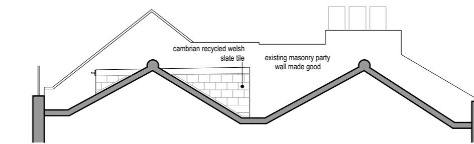
Proposed Elevation AA
