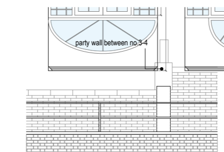
Proposed Elevation BB
