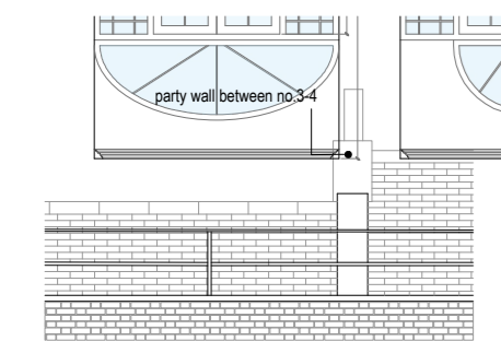
Existing Elevation BB
