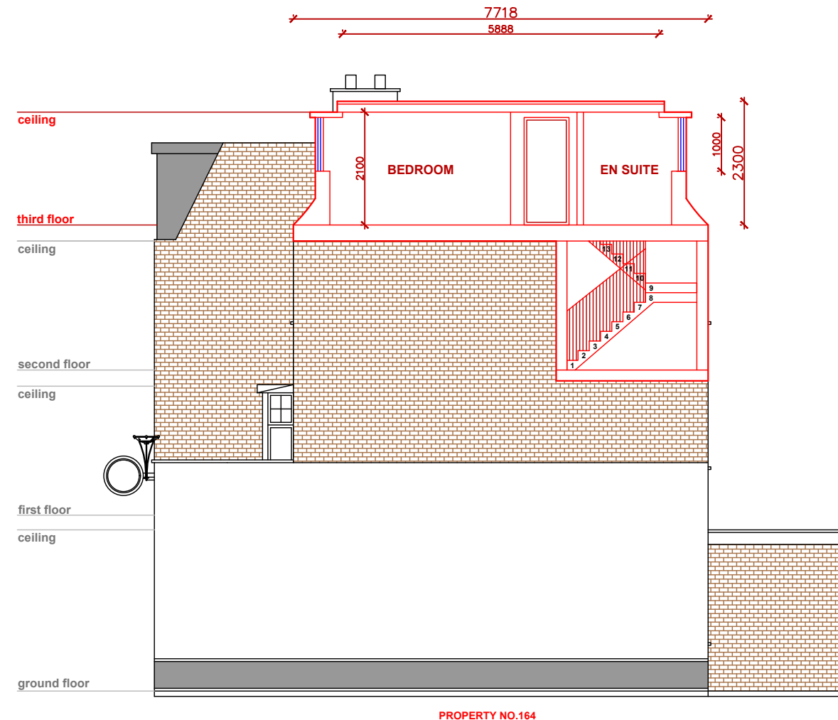
15 PROPOSED SECTION 1:100 @A3
