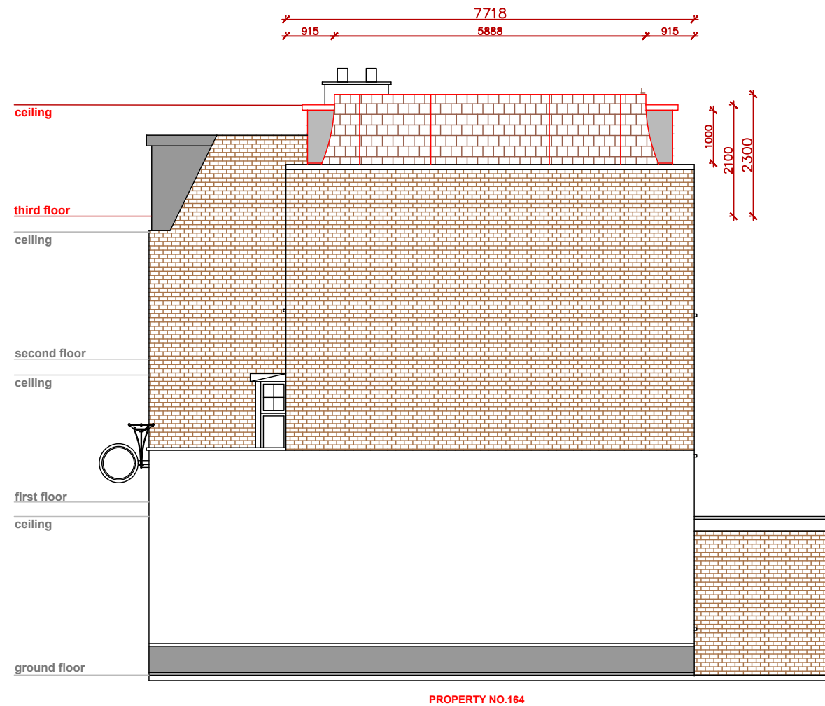
14 PROPOSED SIDE ELEVATION 1:100 @A3
