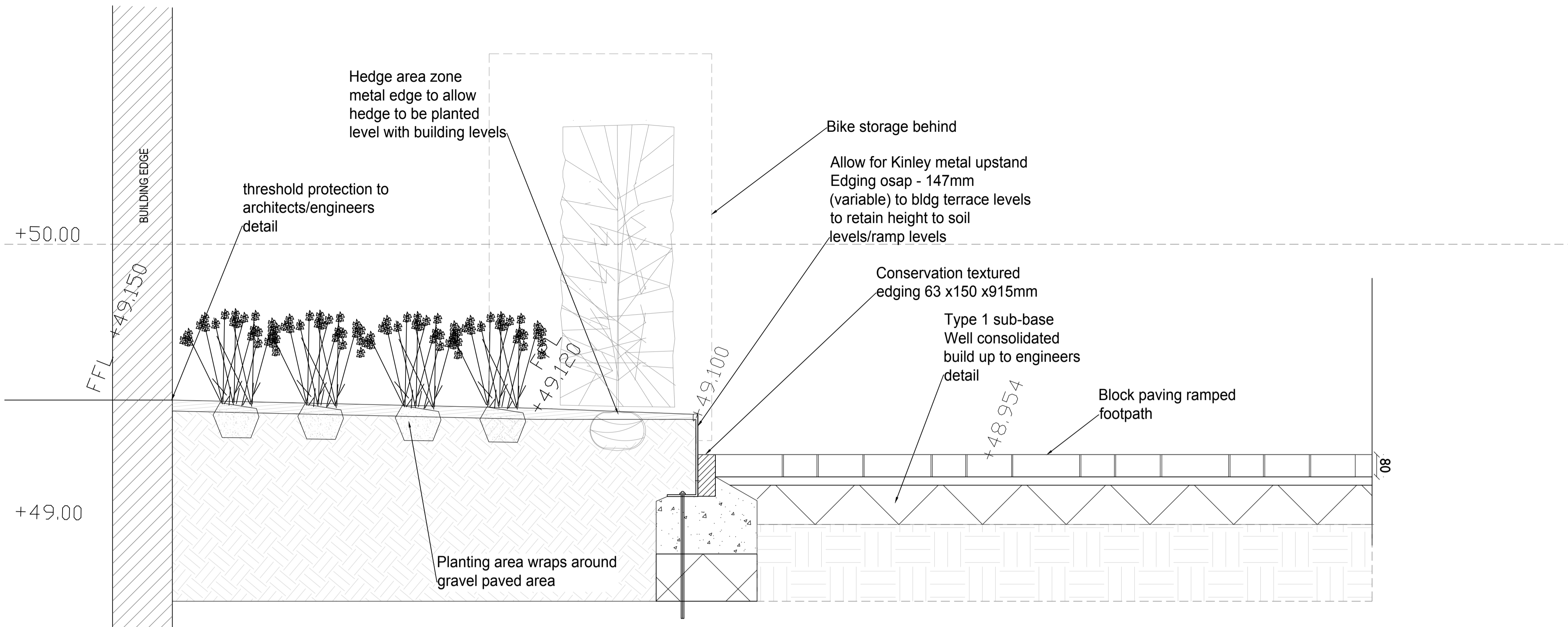
01 Block C front planting: section G-G (levels vary along building frontage) Scale 1:10
