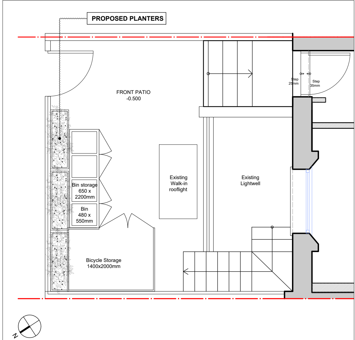
3 PROPOSED FRONT GARDEN PLAN
