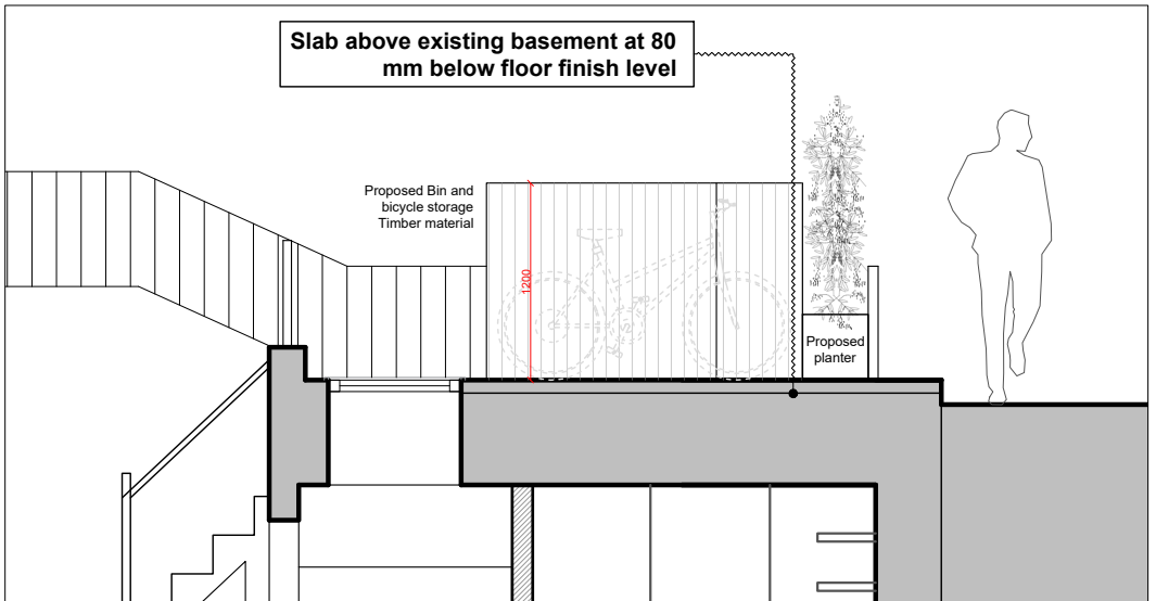
6 PROPOSED SIDE VIEW
