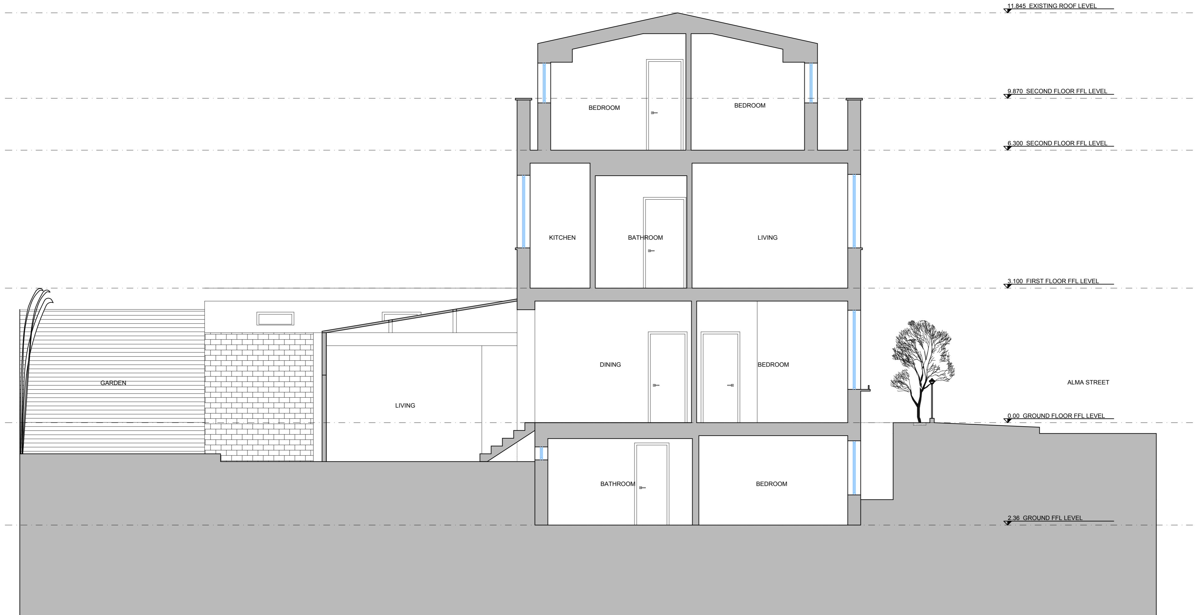
10 Existing section AA -176 Scale 1:50
