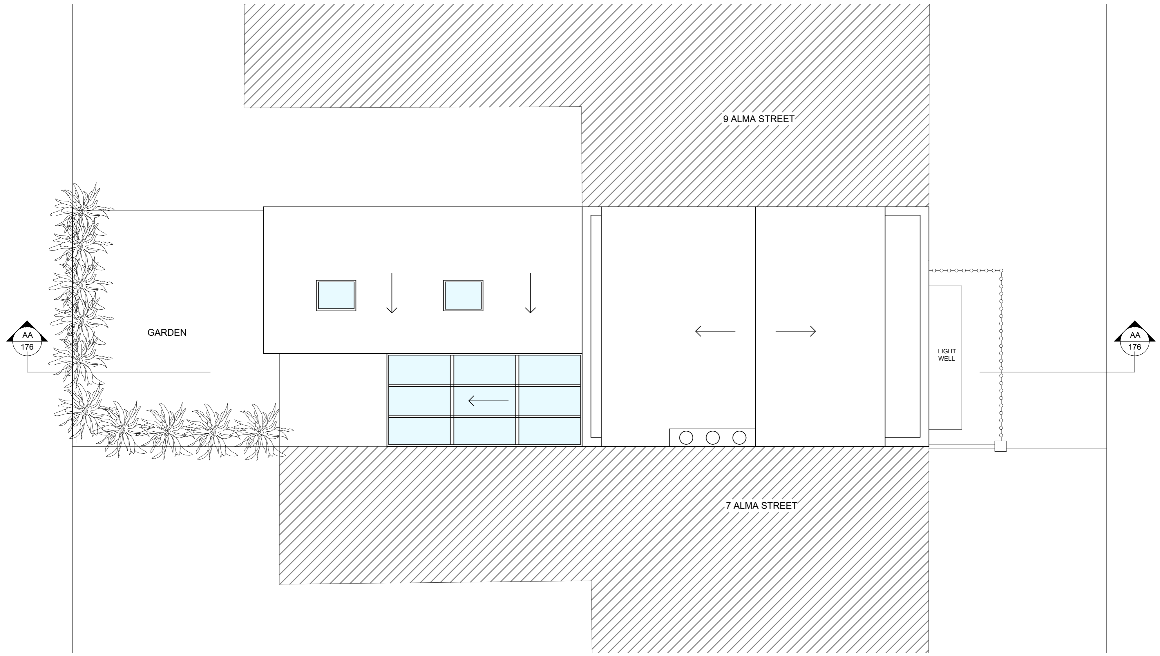
07 Existing roof plan Scale 1:50
