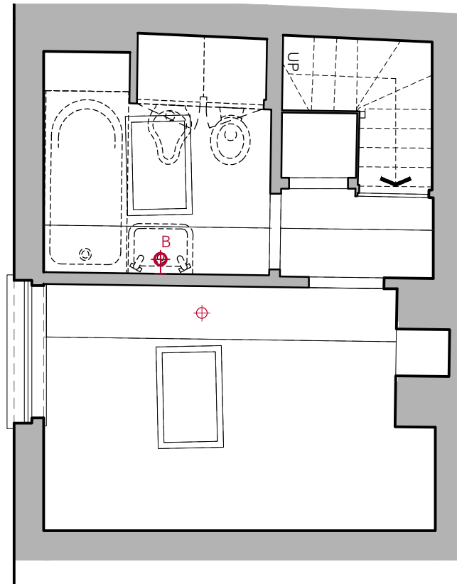
1 EXISTING SECOND FLOOR RCP LIGHTING PLAN Scale 1:20
