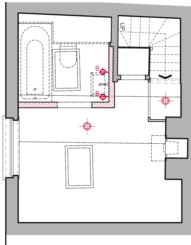
2 PROPOSED SECOND FLOOR RCP LIGHTING PLAN Scale 1:20
