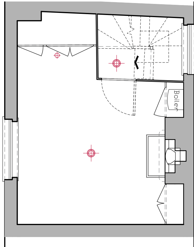
1 EXISTING FIRST FLOOR RCP LIGHTING PLAN Scale 1:20
