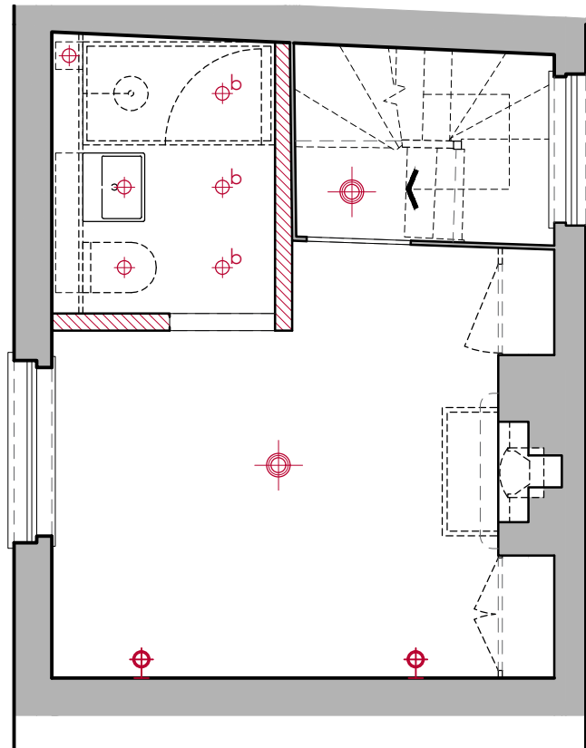
2 PROPOSED FIRST FLOOR RCP LIGHTING PLAN Scale 1:20
