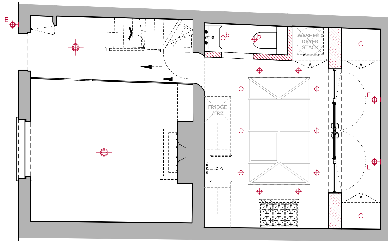
2 PROPOSED GROUND FLOOR RCP LIGHTING PLAN Scale 1:20
