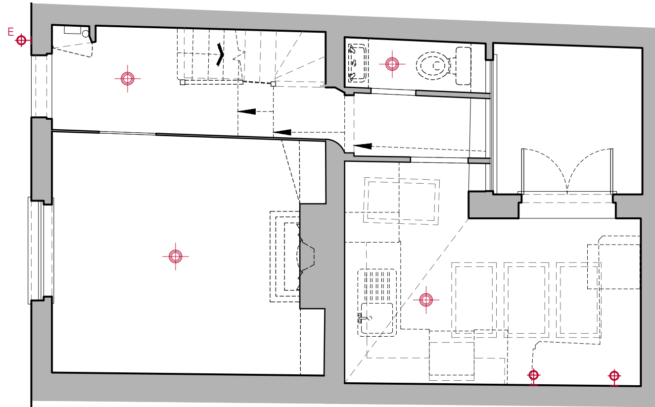
1 EXISTING GROUND FLOOR RCP LIGHTING PLAN Scale 1:20
