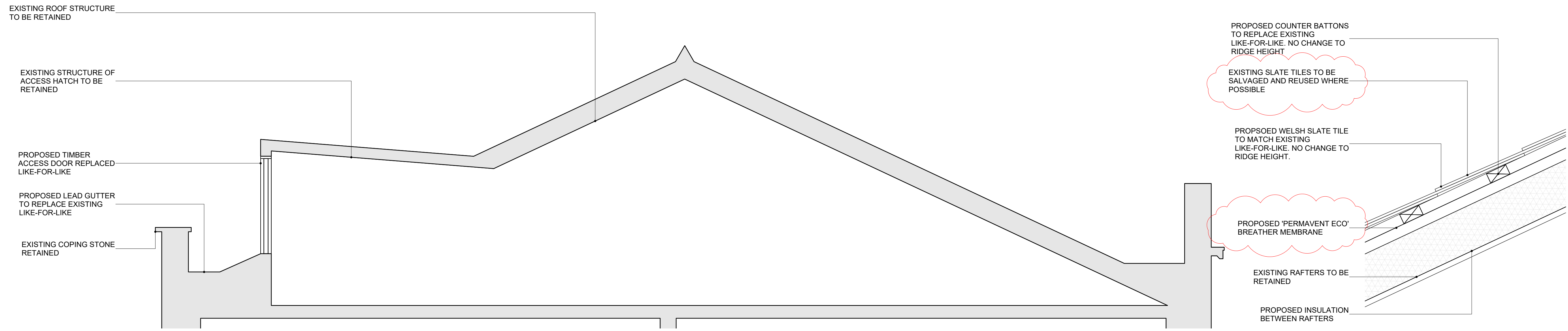
03 ROOF SECTION DETAILS 1:20 @ A1
