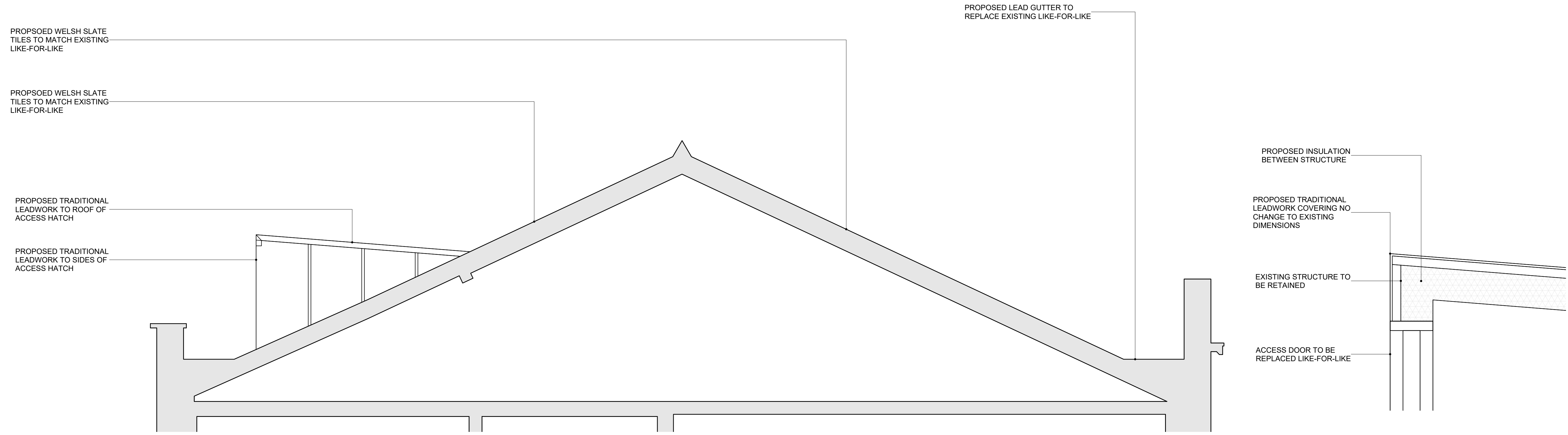
01 ROOF ELEVATION DETAILS 1:20 @ A1
