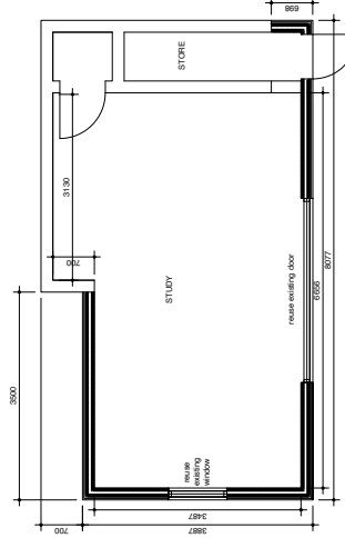
PROPOSED GROUND PLAN
