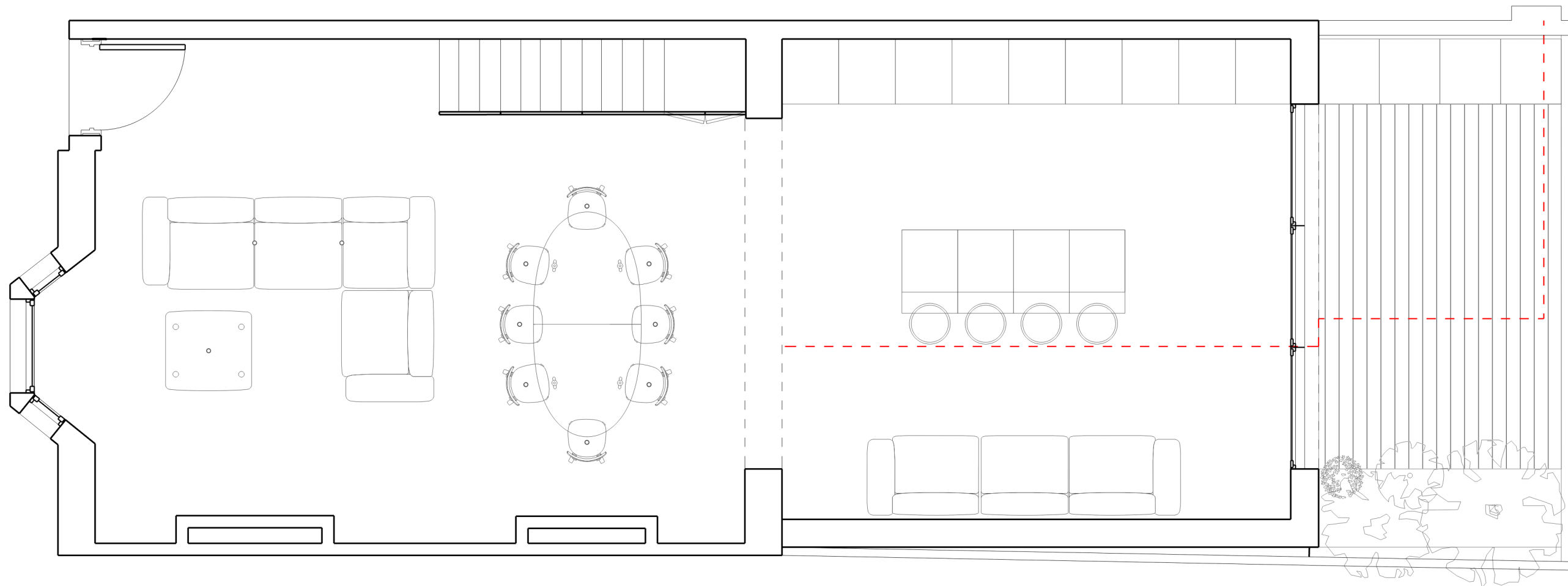
01 Proposed ground floor 1:50
