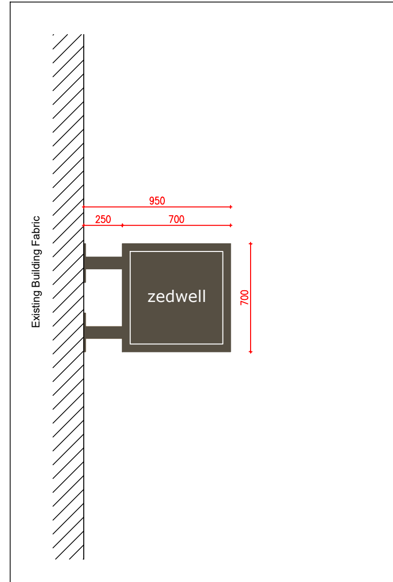
3 Proposed External Sign 2 (Projecting) Section / Elevation 1:25 @ A1 1:50 @ A3
