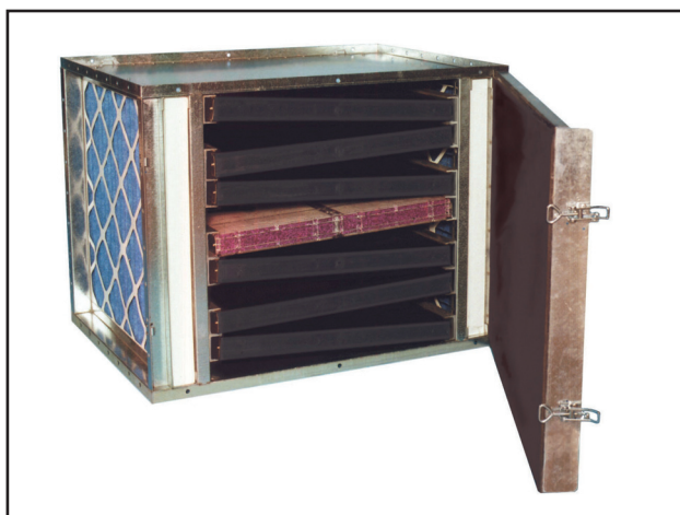
AAC Swiftpack® unit containing PR filters and single AAC Colourcell® filter.
